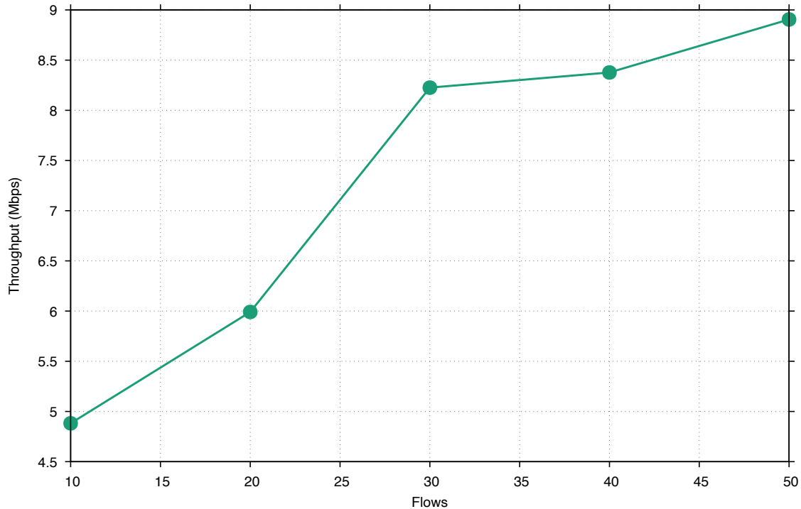
Wired Bolt Throughput (Mbps) vs Flows
