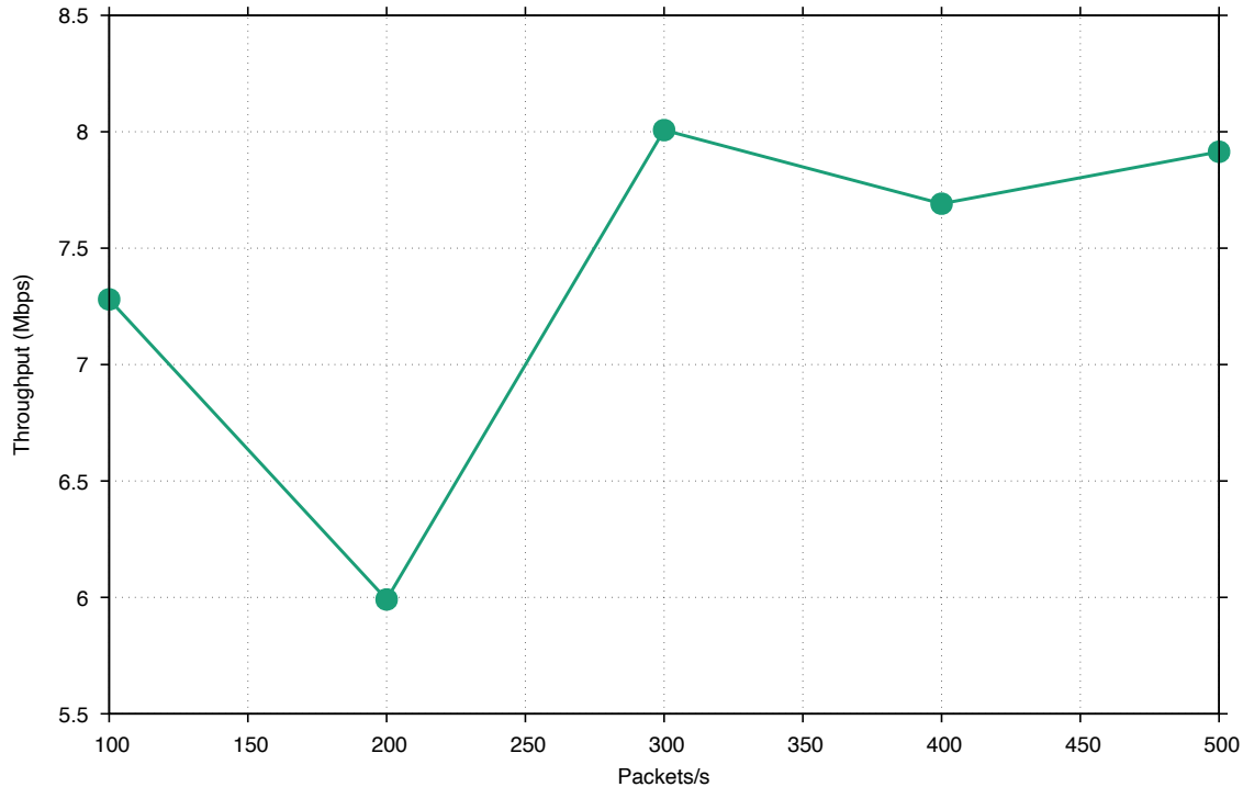
Wired Bolt Throughput (Mbps) vs Packets/s
