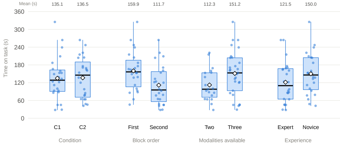
Time on task per observation: box = median and quartiles, diamond = mean
