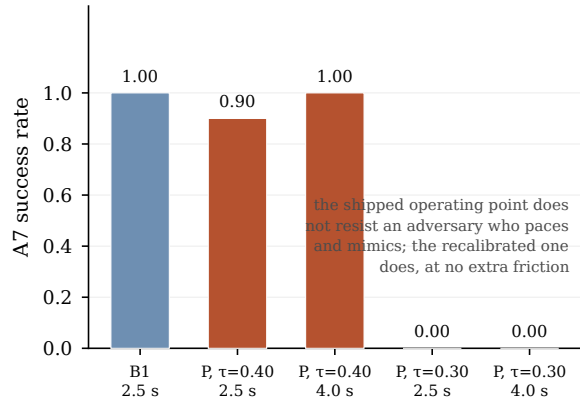
(b) the adaptive adversary
