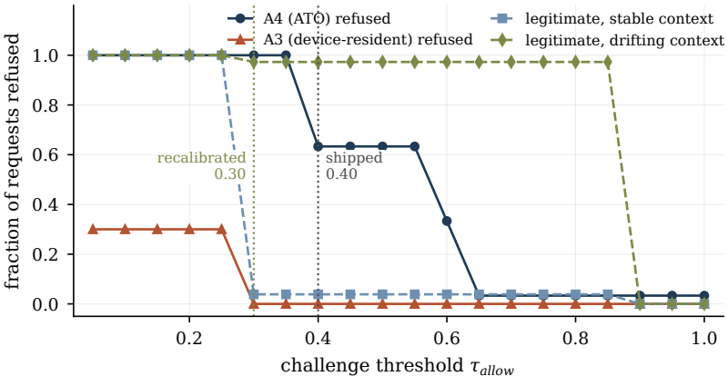
(a) decisions recomputed over the measured risk scores
