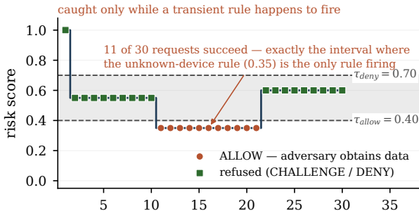
(a) A4 — adversary makes no attempt to evade
