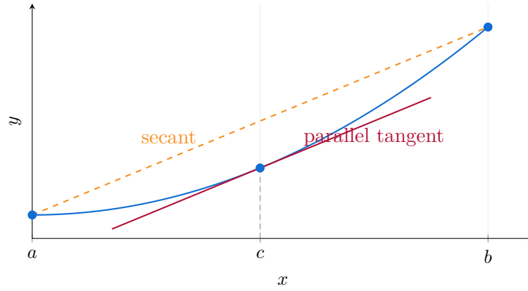
Figure 5.3: An exact MVT example: f(x) = 0.2x^2 + 0.4 on [0, 4] . The secant slope is 0.8 = f'(2) .
