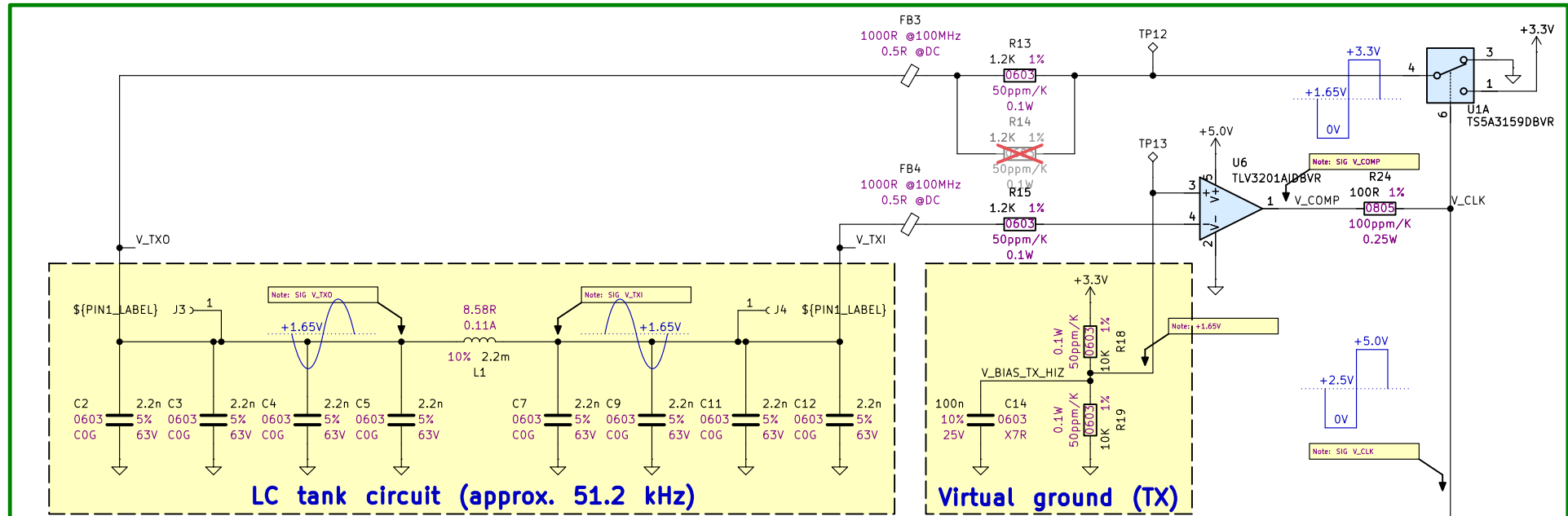
TX Circuit
