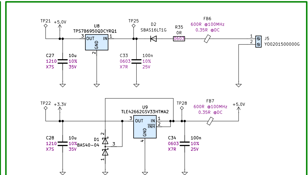
+5V / +3.3V power supply
