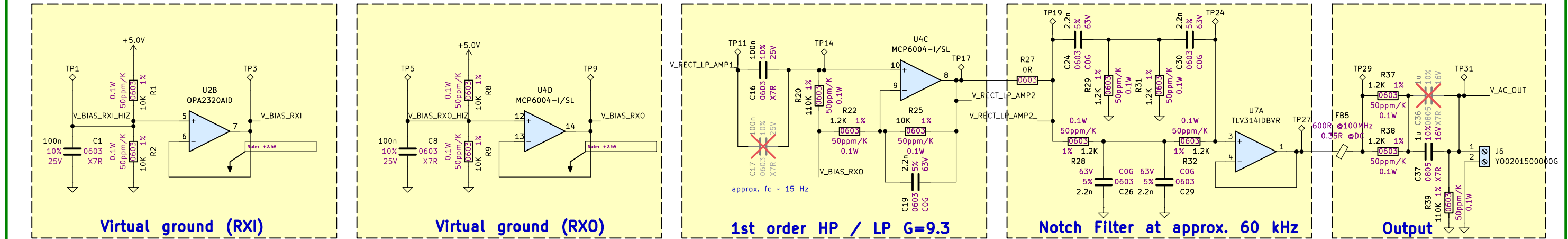
RX Circuit
