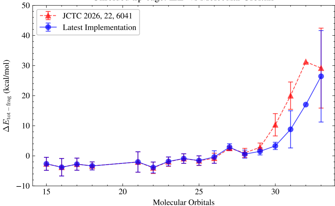
Unfolded trp-cage: \Delta E vs Molecular Orbitals
