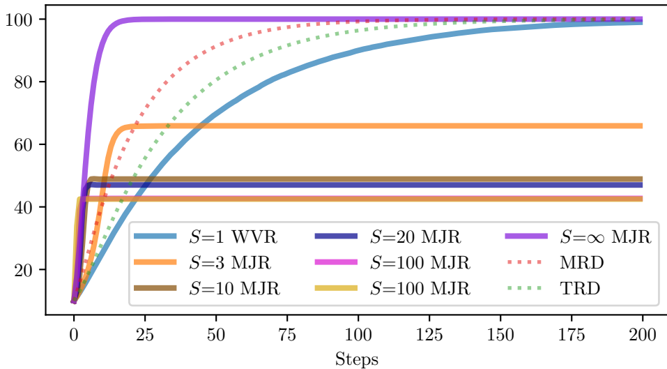
Average % optimal action
