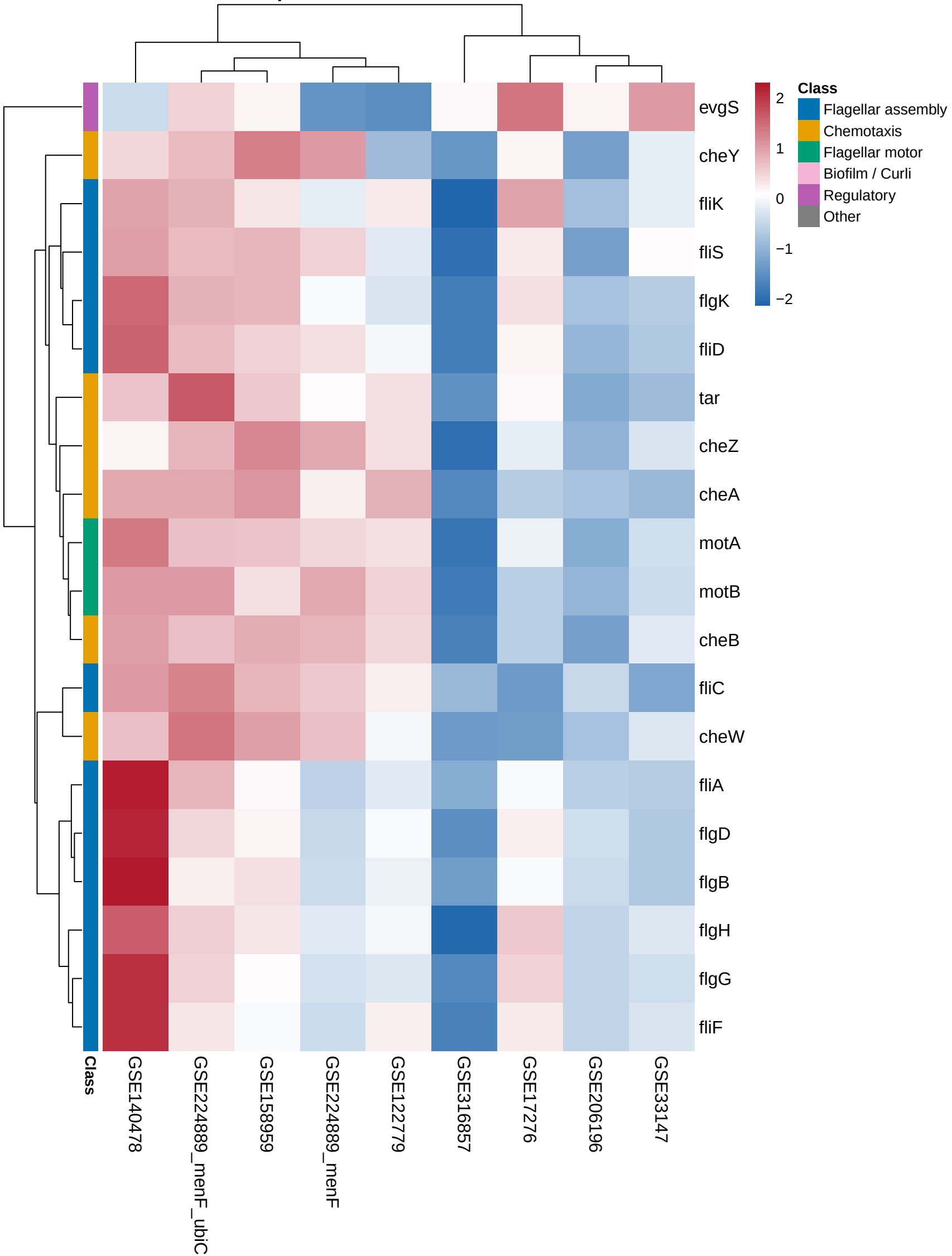
Hub Gene Expression Patterns Across ALE Datasets
