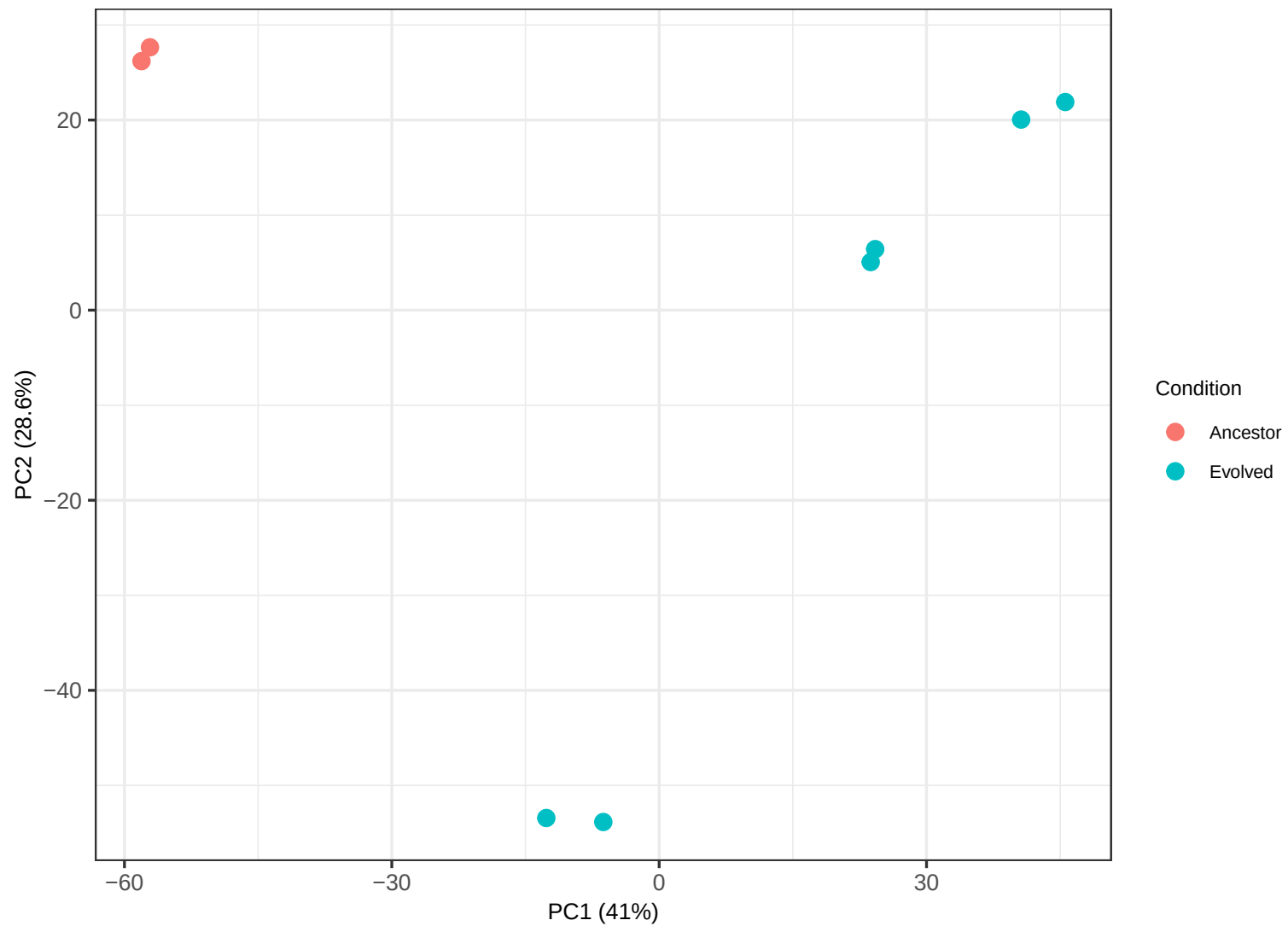
PCA of log expression values (Evolved vs Ancestor, GSE122779)
