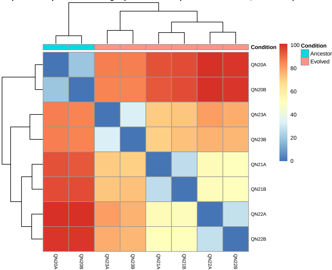
Sample-to-Sample Distance of log expression values (Evolved vs Ancestor, GSE122779)
