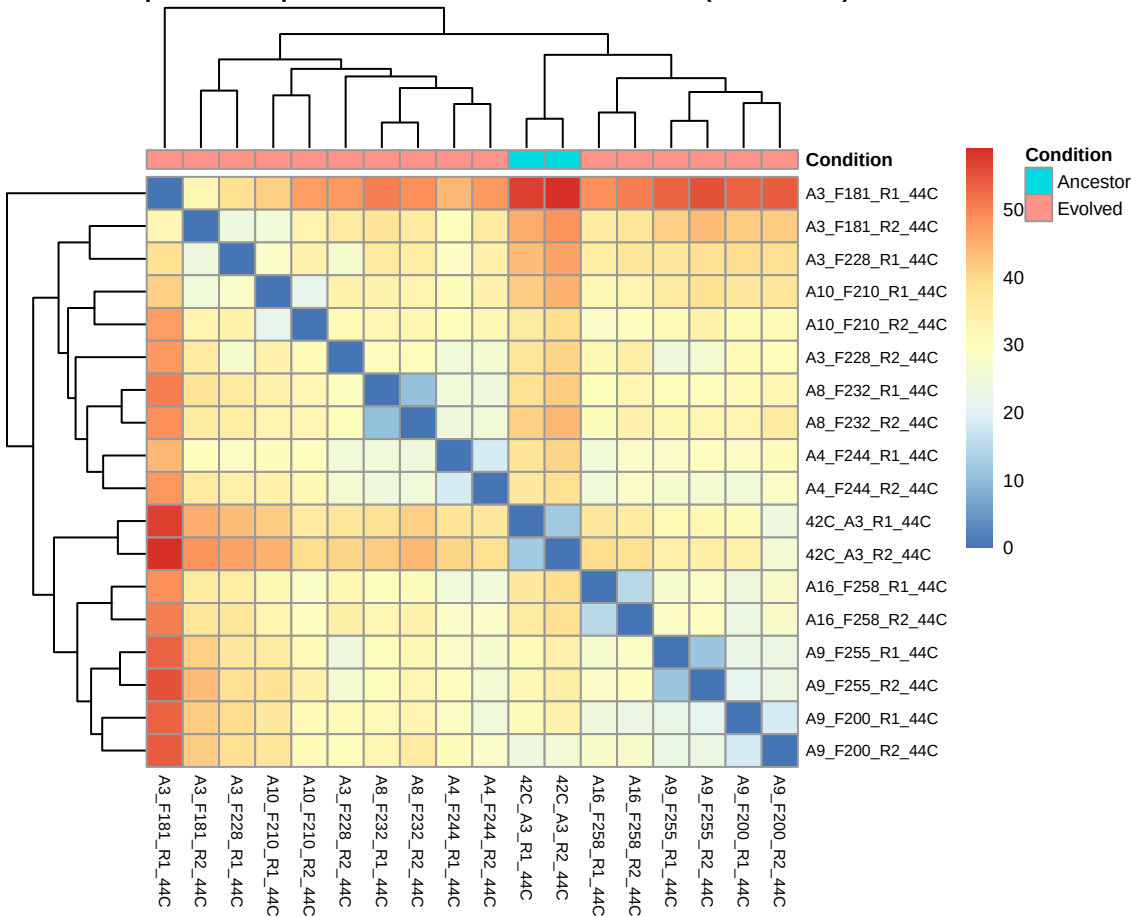
Sample-to-Sample Distance after VST normalization (GSE140478)
