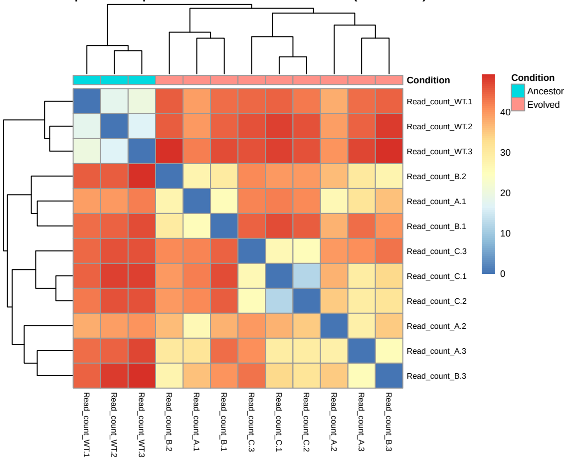
Sample-to-Sample Distance after VST normalization (GSE158959)
