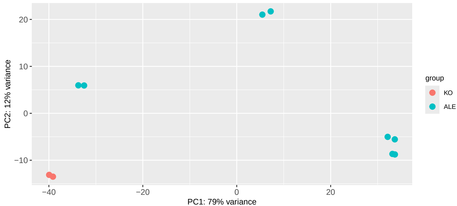
PCA of VST-normalized counts-menF-ubiC (GSE224889)
