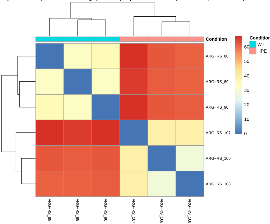
Sample-to-Sample Distance of \log_2(\text{TPM} + 1) expression values (HPE vs WT, GSE316857)
