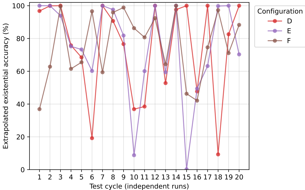
Extrapolated Existential Accuracy Across Independent Test Cycles for Different Configurations
