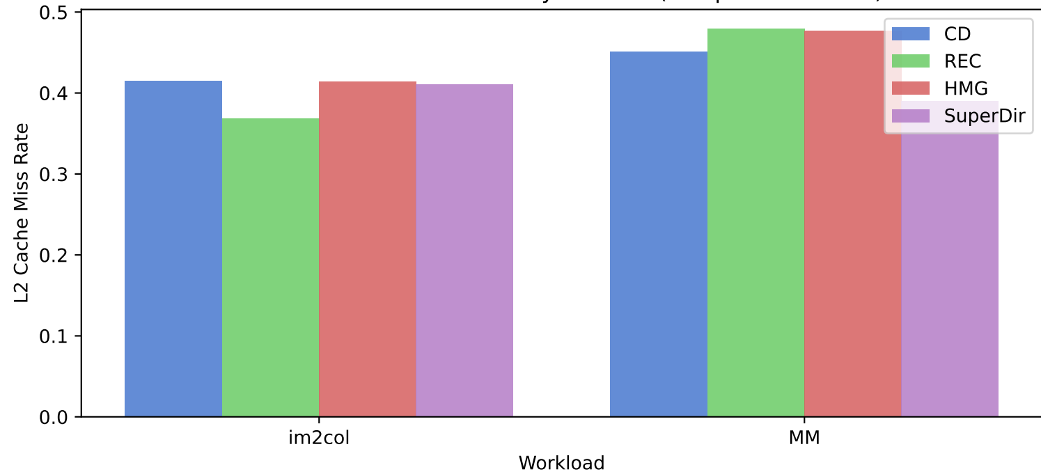
F-P3: L2 Cache Miss Rate by Scheme (compute GPUs 2-5)
