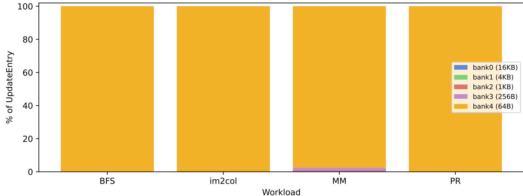
F-P4: SuperDir Bank Utilization (region size distribution) WARNING: 97-99% in bank4 (64B) — adaptation NEVER triggered
