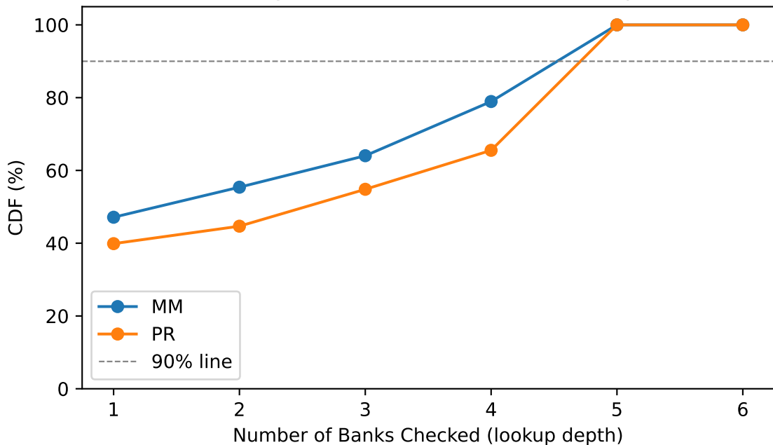
F-P6: SuperDir BankChecked CDF Note: avg MM=2.55, PR=2.95 banks/request
