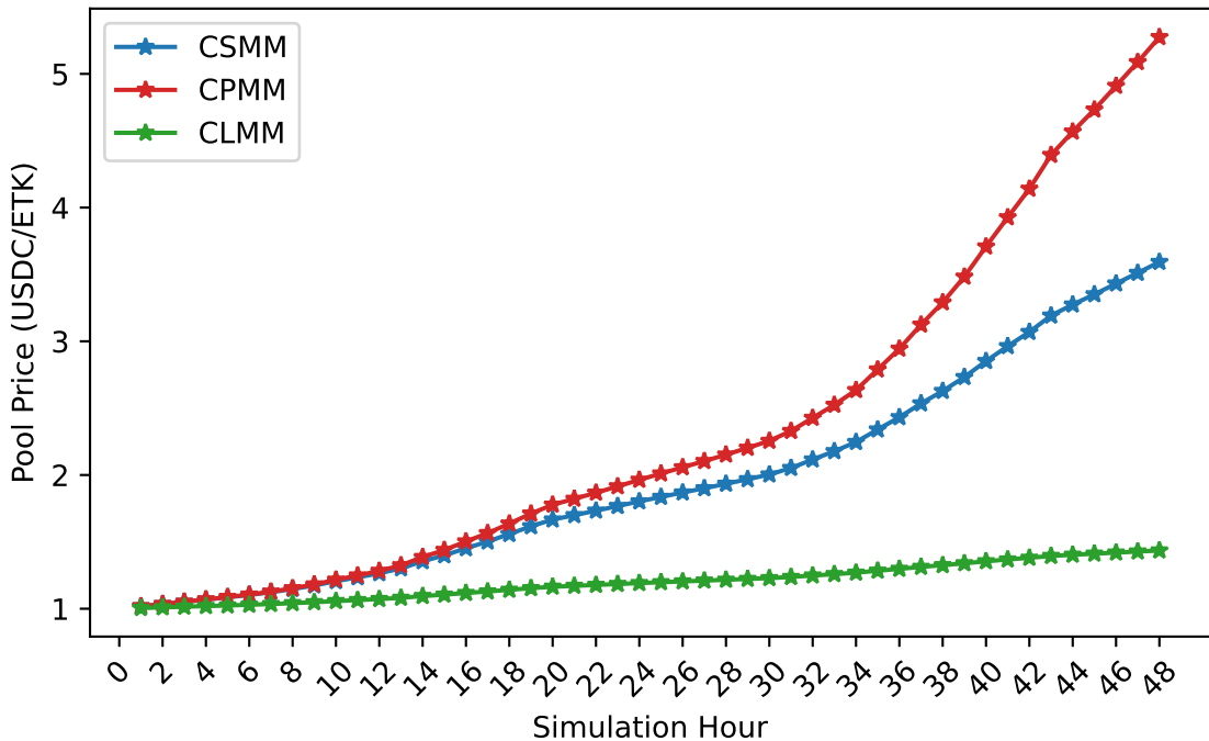
EnergyAMM Simulation Curve Comparison
