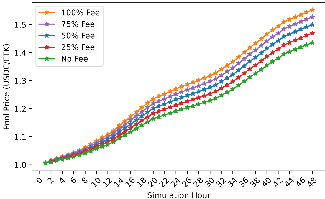
EnergyAMM Simulation CLMM Fee Rate Comparison
