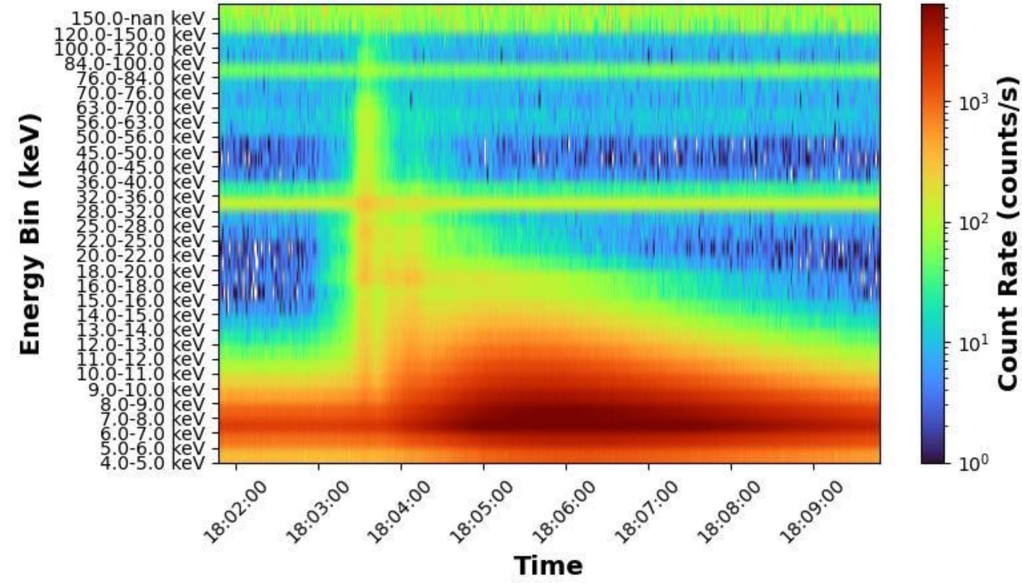
STIX Count Rate Spectrogram of Event-5
