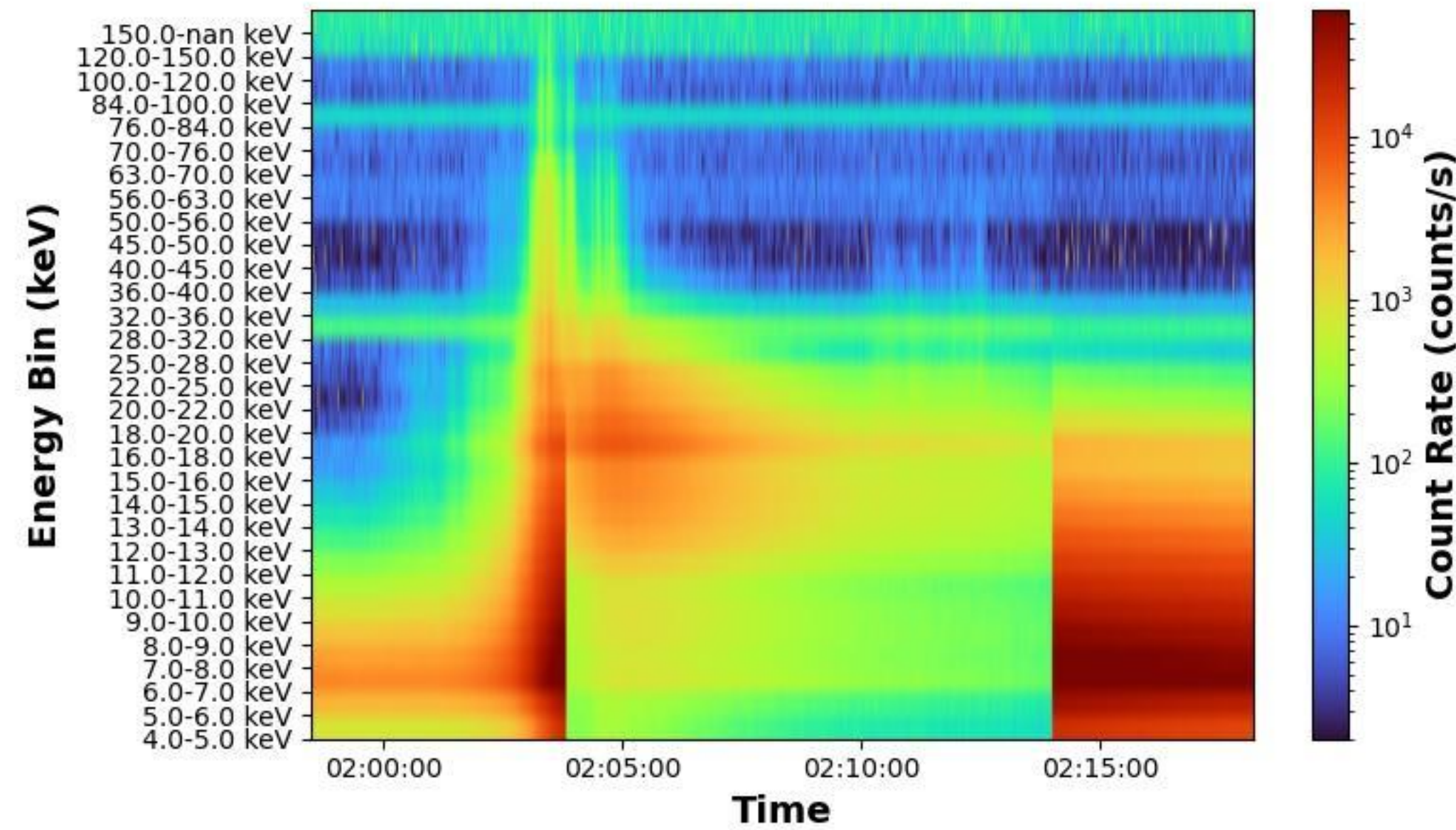
STIX Count Rate Spectrogram of Event-2
