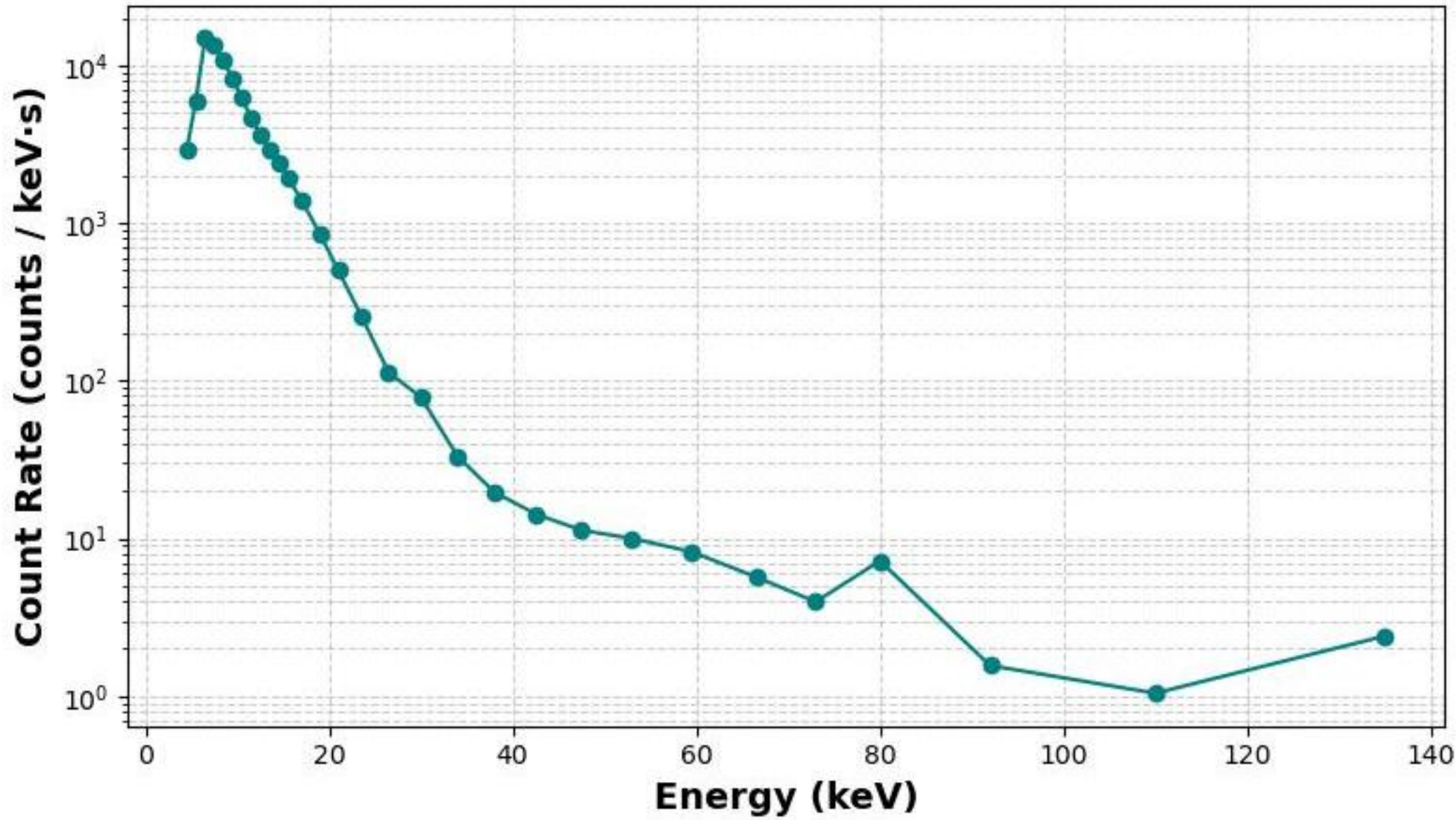
X-ray Energy Spectrum of Event-3 from 15:18:00 to 15:20:00
