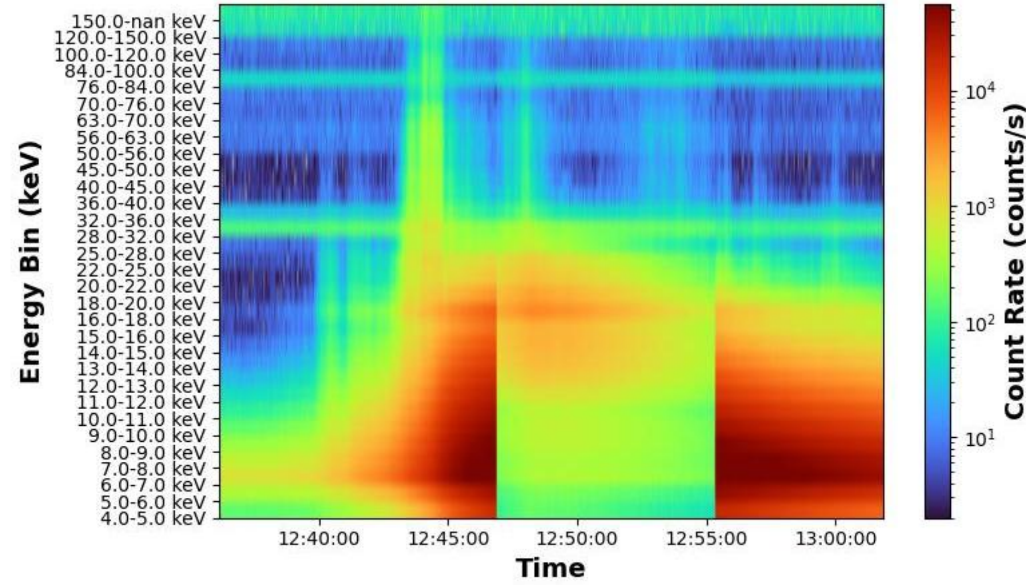
STIX Count Rate Spectrogram of Event-3
