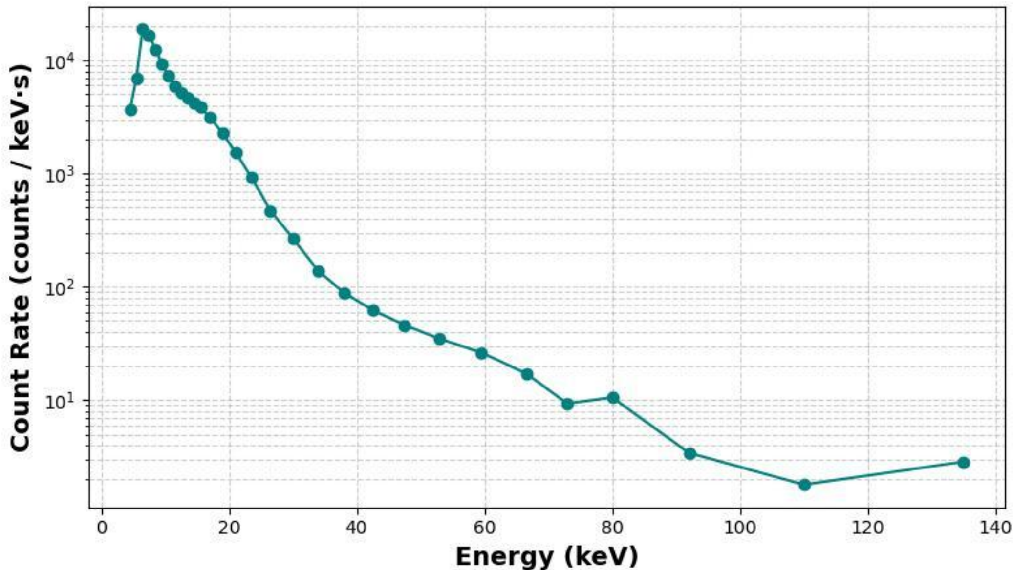
X-ray Energy Spectrum of Event-2 from 12:42:00 to 12:52:00
