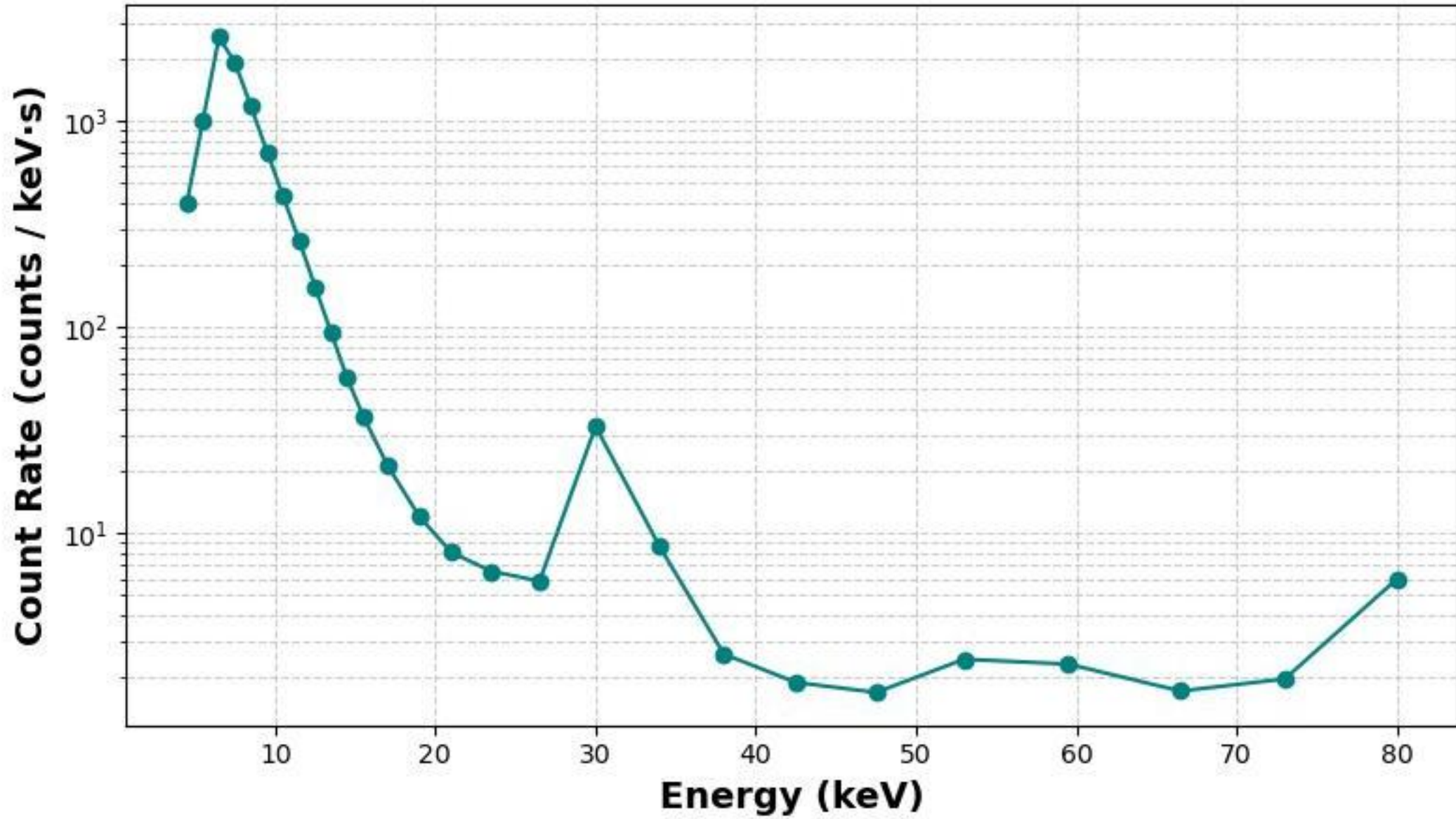
X-ray Energy Spectrum of Event-4 from 16:43:00 to 16:51:00
