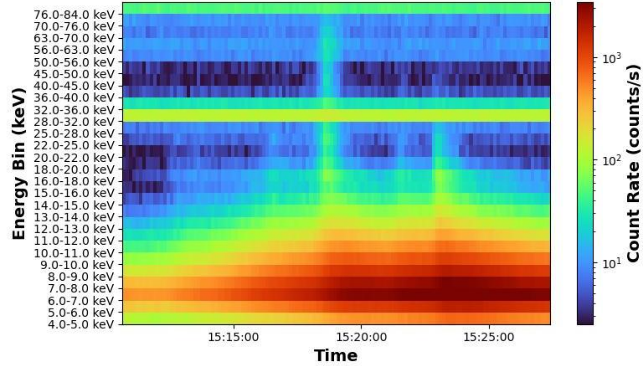
STIX Count Rate Spectrogram of Event-4
