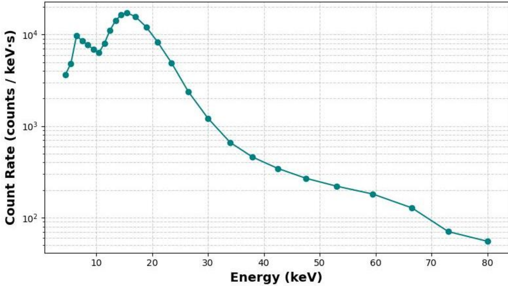
X-ray Energy Spectrum of Event-5 from 18:03:00 to 18:04:00
