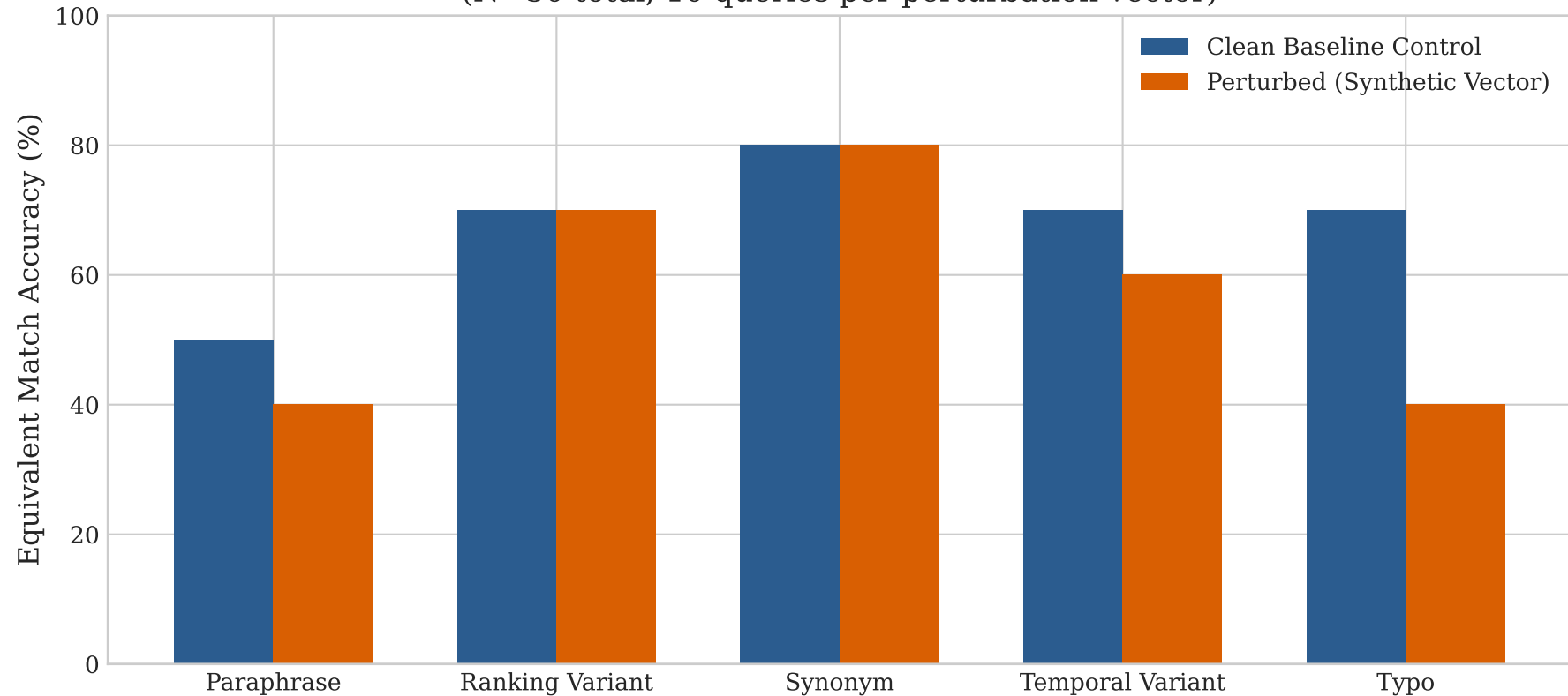
Figure 6: Robustness Under Controlled Synthetic Perturbations (N=50 total; 10 queries per perturbation vector)
