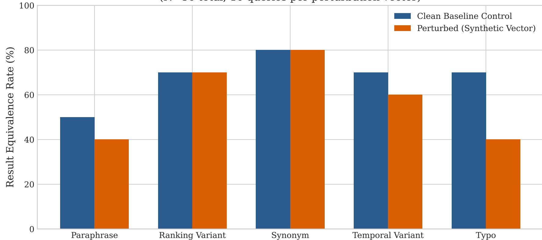
Robustness Under Controlled Synthetic Perturbations (N=50 total; 10 queries per perturbation vector)
