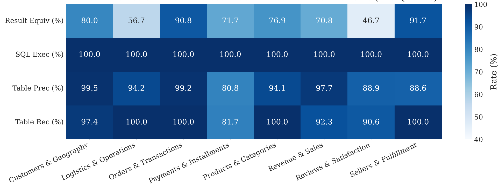
Performance Stratification Across E-Commerce Business Domains (500 Queries)
