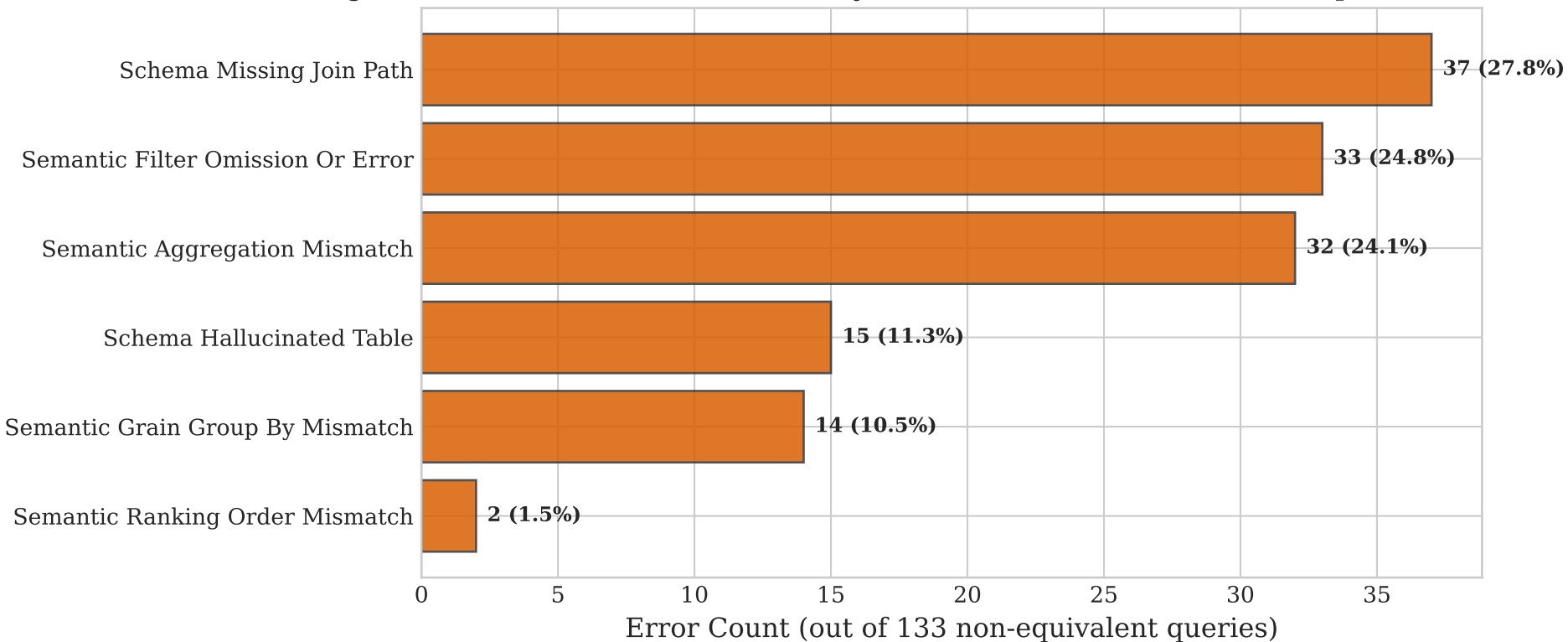
Figure 7: Scientific Failure Taxonomy Distribution across 133 Non-Equivalent Queries
