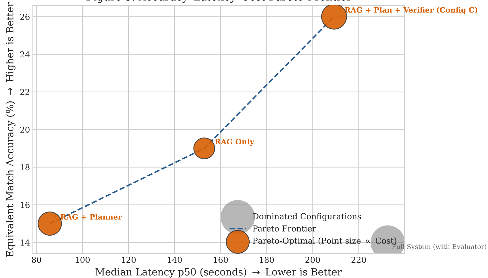
Figure 3: Accuracy-Latency-Cost Pareto Frontier
