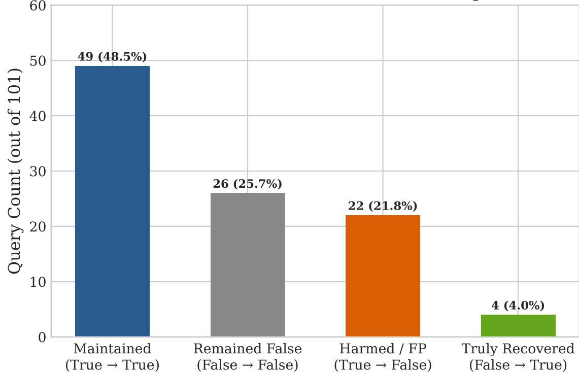
(B) Semantic Transitions (Pre \rightarrow Post Repair)
