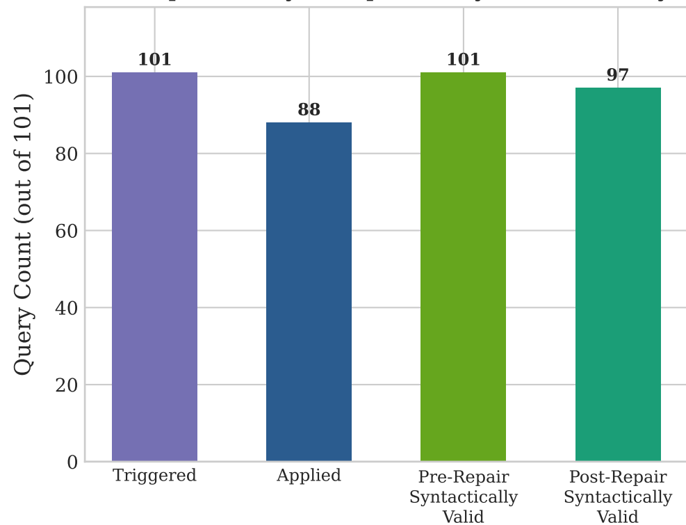
(A) Repair Lifecycle Pipeline (Syntactic Validity)
