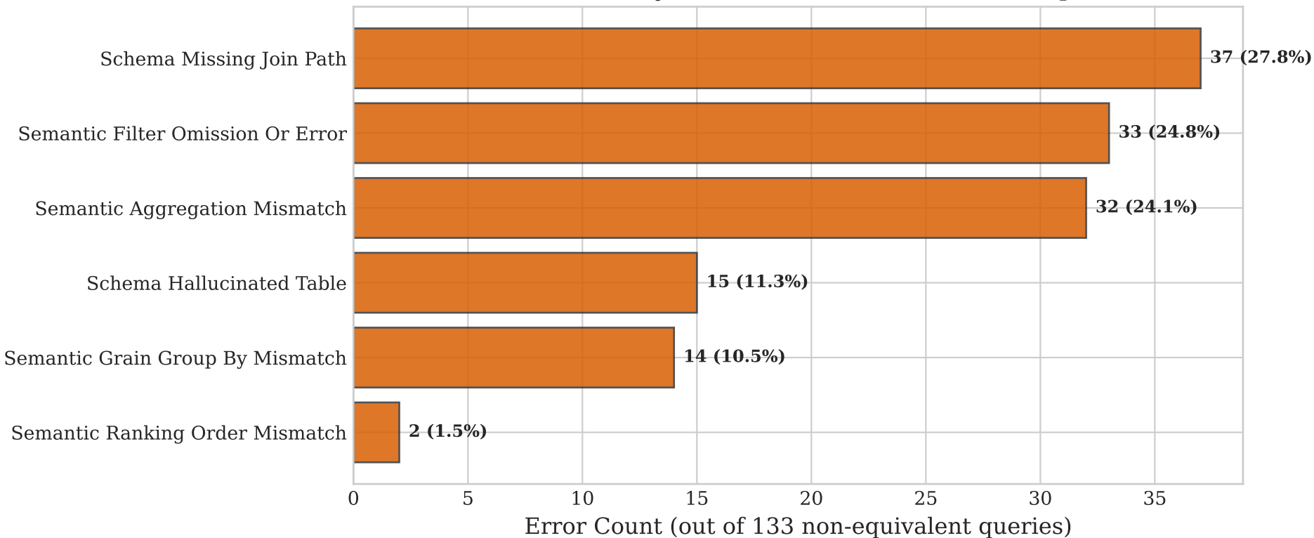
Scientific Failure Taxonomy Distribution across 133 Non-Equivalent Queries
