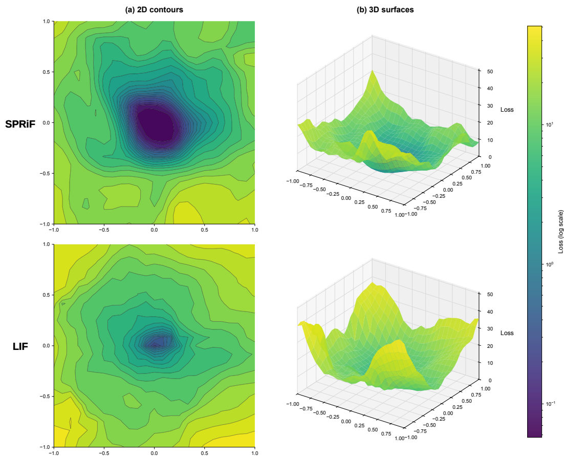
Figure S1: S-MNIST loss-landscape diagnostic for SPRiF (top row) and LIF (bottom row). The 2D contours and 3D surfaces show cross-entropy over the same 25 \times 25 perturbation-coordinate grid, with a shared logarithmic color scale and common vertical range. Each model uses its own checkpoint-normalized random directions, while evaluation samples and grid coordinates are matched.
