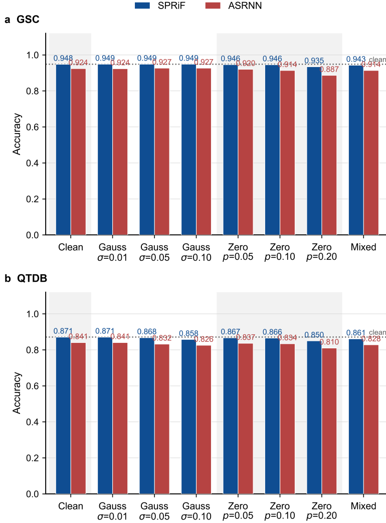
Figure S3: Feature-space perturbation diagnostic using saved checkpoints. SPRiF and ASRNN are evaluated on GSC and QTDB under additive Gaussian noise, random feature zeroing, and mixed perturbations. The clean values in this diagnostic come from the saved checkpoints used for the perturbation sweep and need not equal the five-seed benchmark summaries in the main paper.
