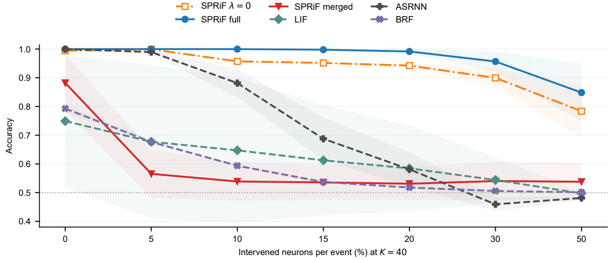
Figure S2: SI-DMS fraction response at the unseen intervention count K = 40 . Curves are 3-seed means after averaging each seed over five delays; shaded bands show seed standard deviations. The point at 0% is the clean condition, and 15% is the intervention fraction used during training.
