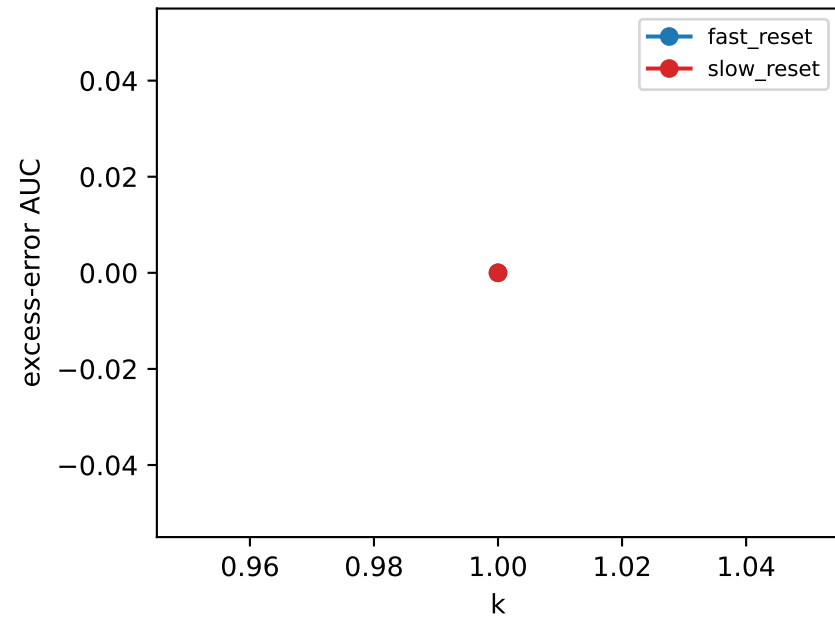
K sensitivity
