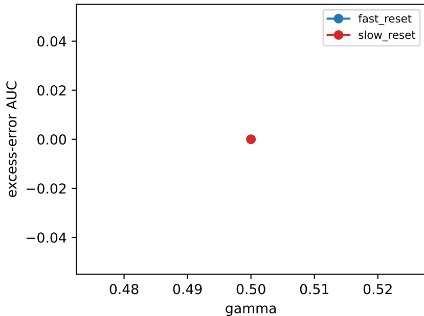
Reset-strength sensitivity
