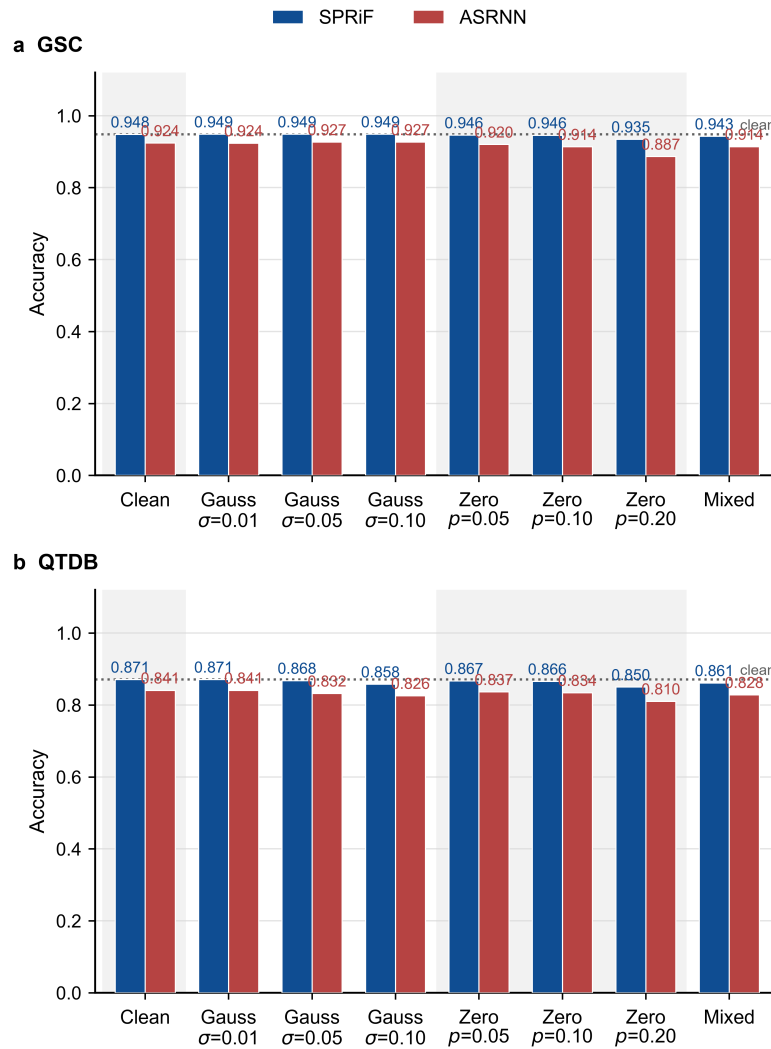
Figure S2: Feature-space perturbation diagnostic using saved checkpoints. SPRiF and ASRNN are evaluated on GSC and QTDB under additive Gaussian noise, random feature zeroing, and mixed perturbations. The clean values in this diagnostic come from the saved checkpoints used for the perturbation sweep and need not equal the five-seed benchmark summaries in the main paper.
