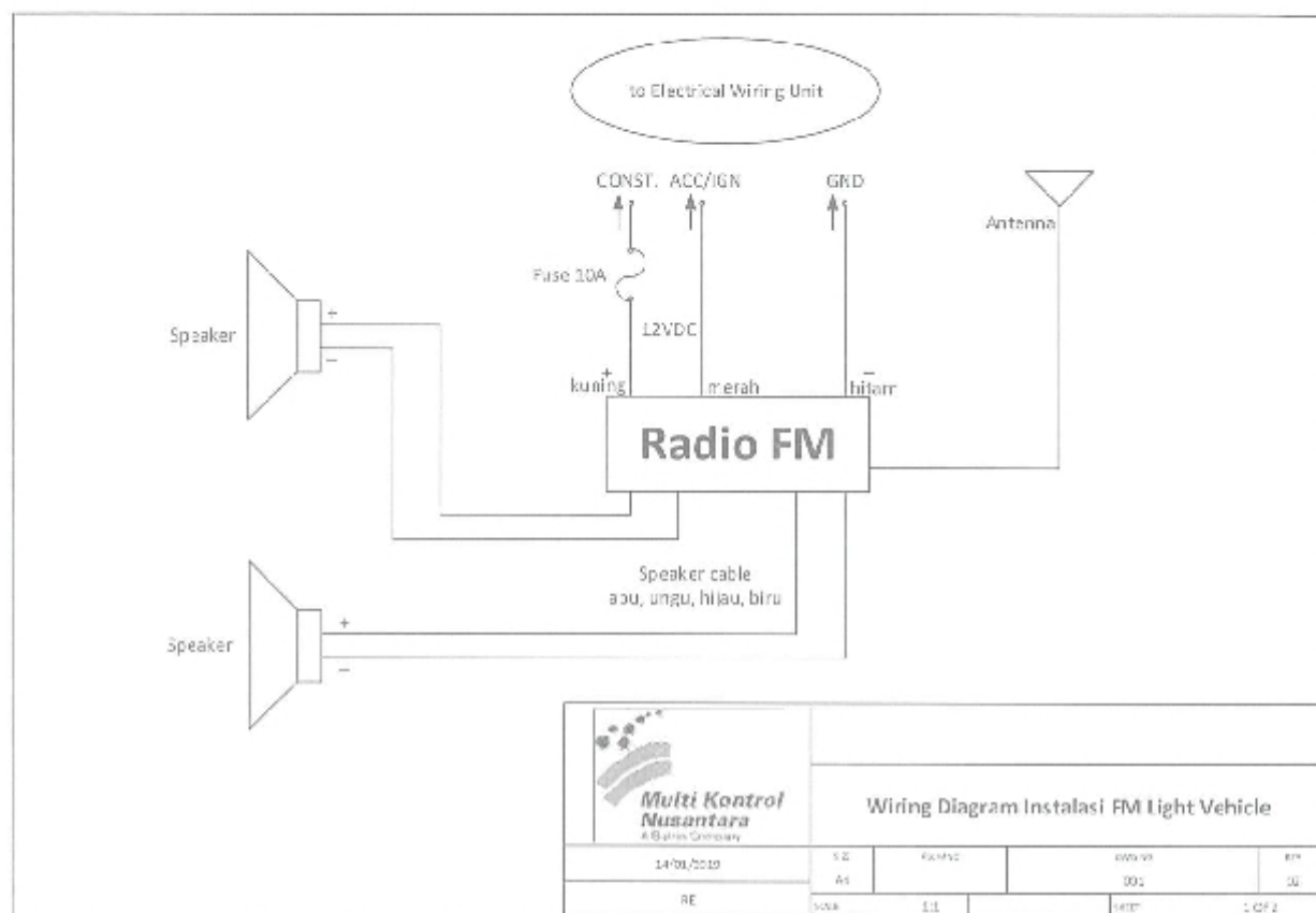
Gh. 1 – Wiring Diagram Instalasi FM Light Vehicle
