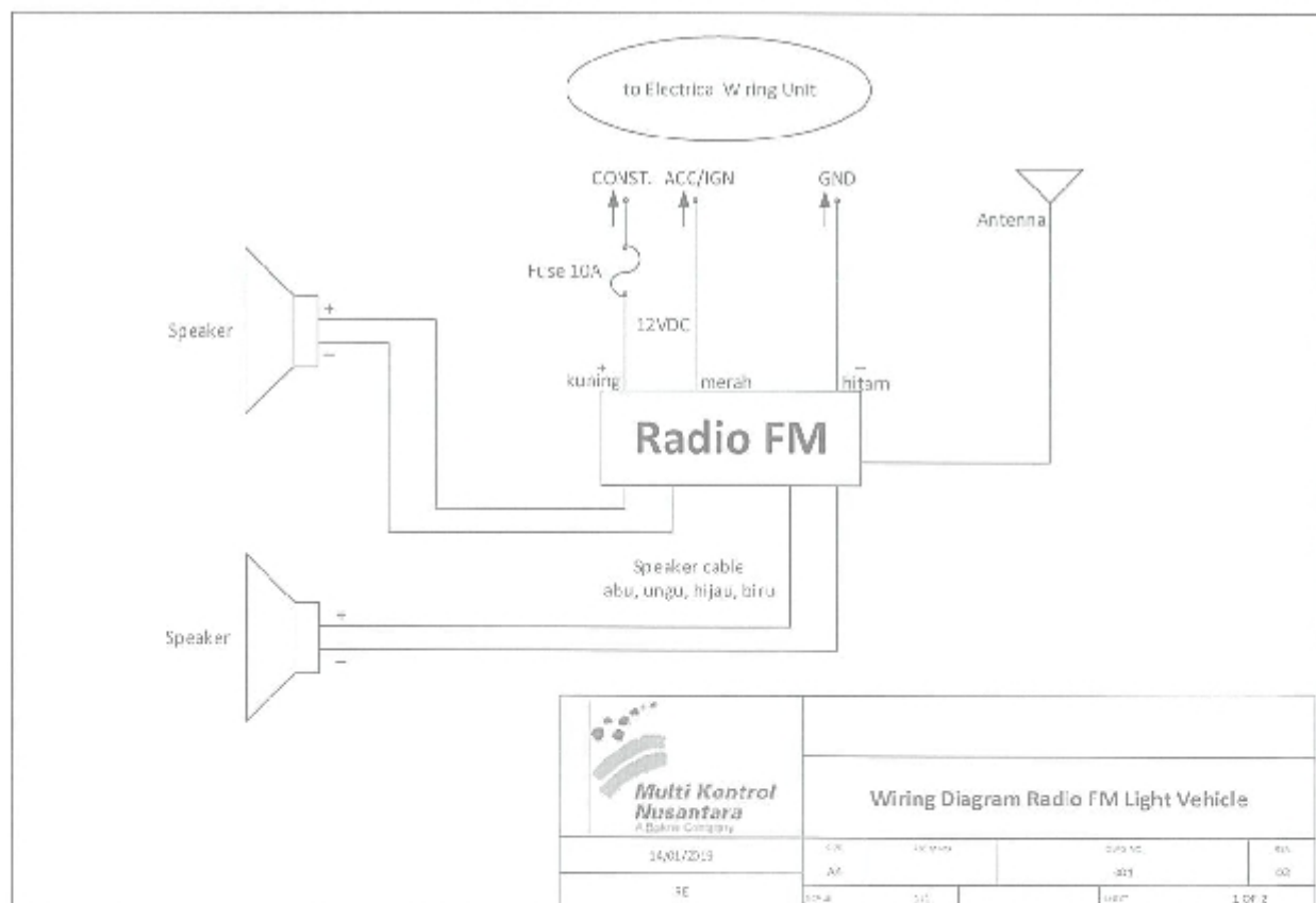
Gb. 1 – Wiring Diagram Radio FM Light Vehicle
