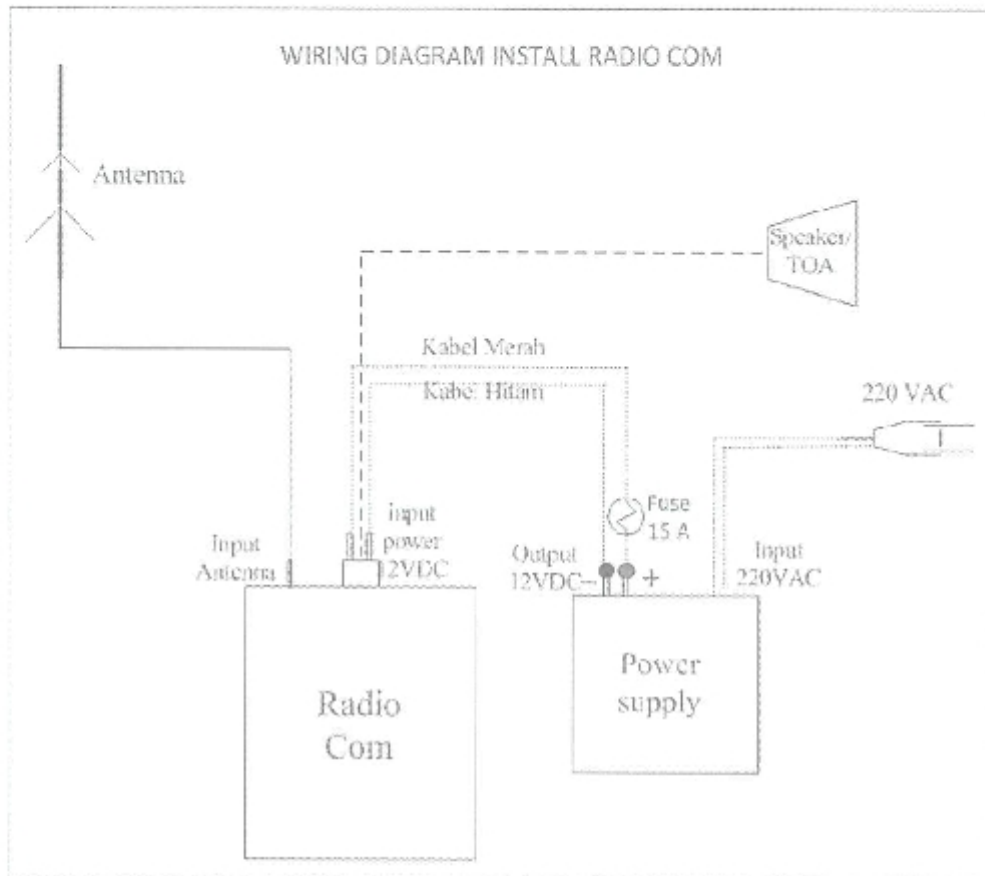
Gb.1- Wiring Diagram Instalasi Radio Komunikasi Di Base Station
