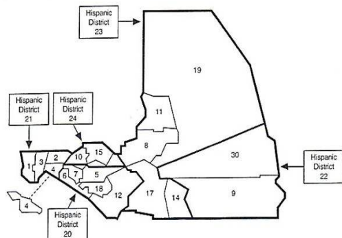
Mid-Southern California Area Districts
