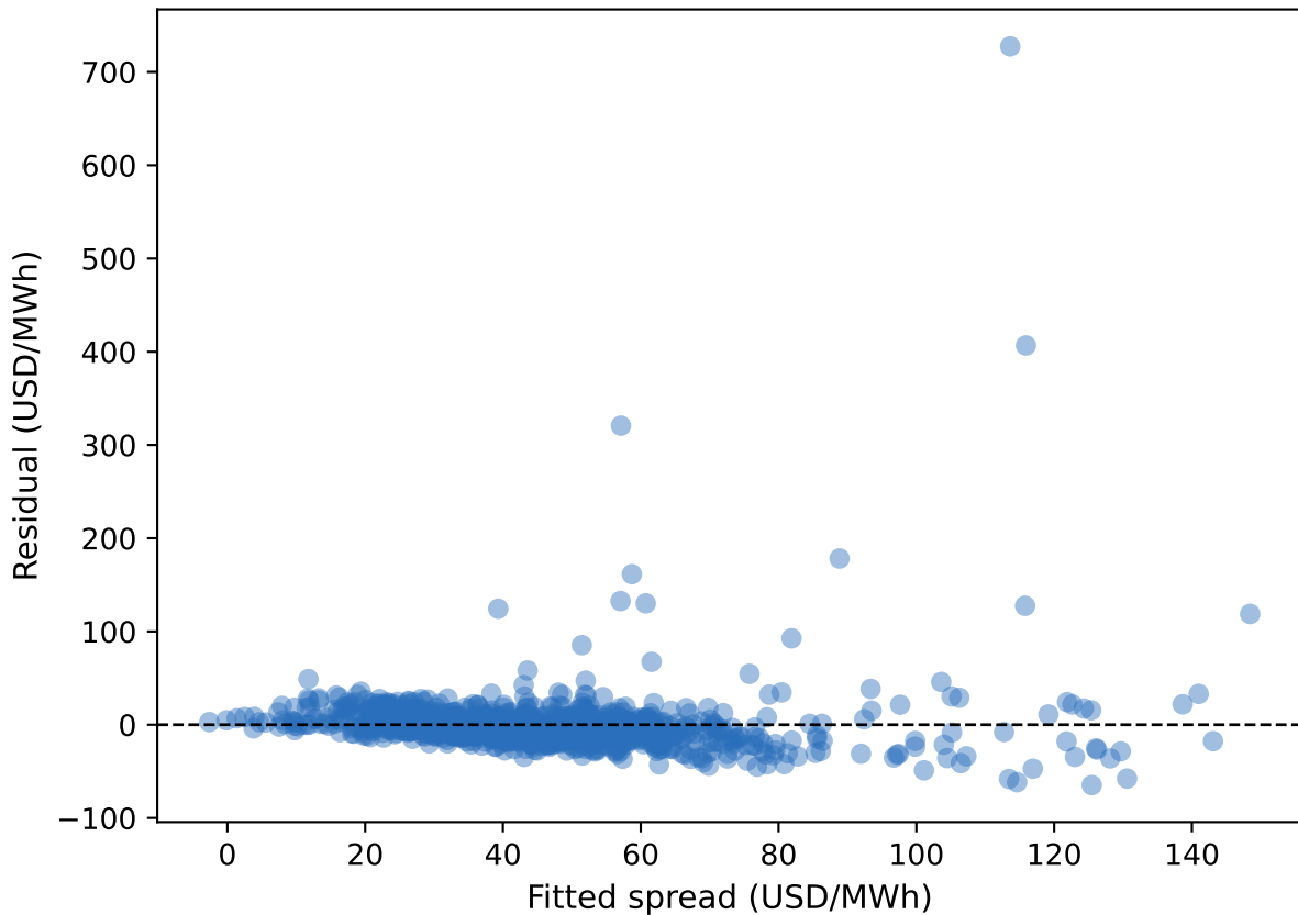
Baseline residuals against fitted values
