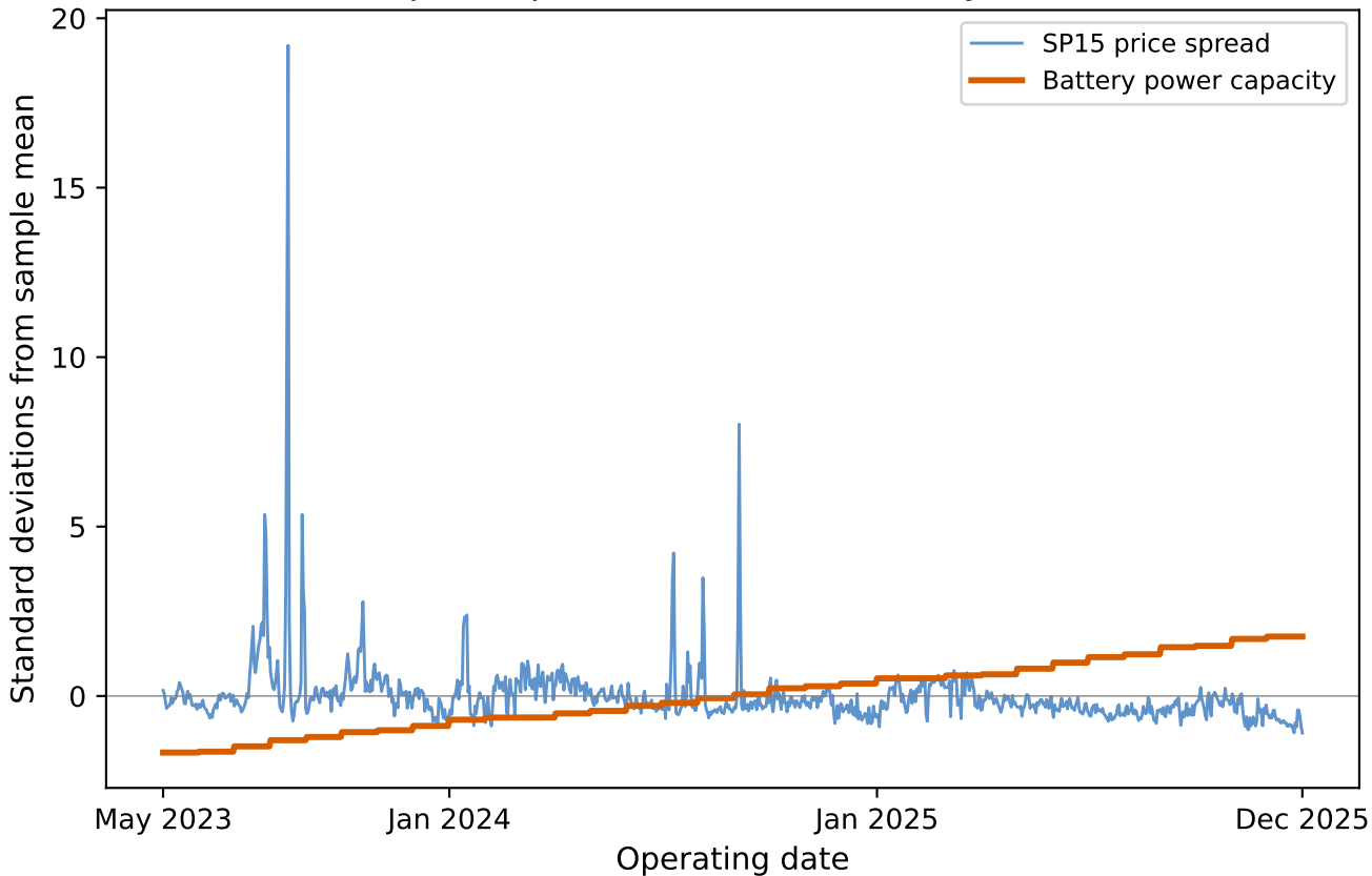
SP15 price spread and CAISO battery build-out
