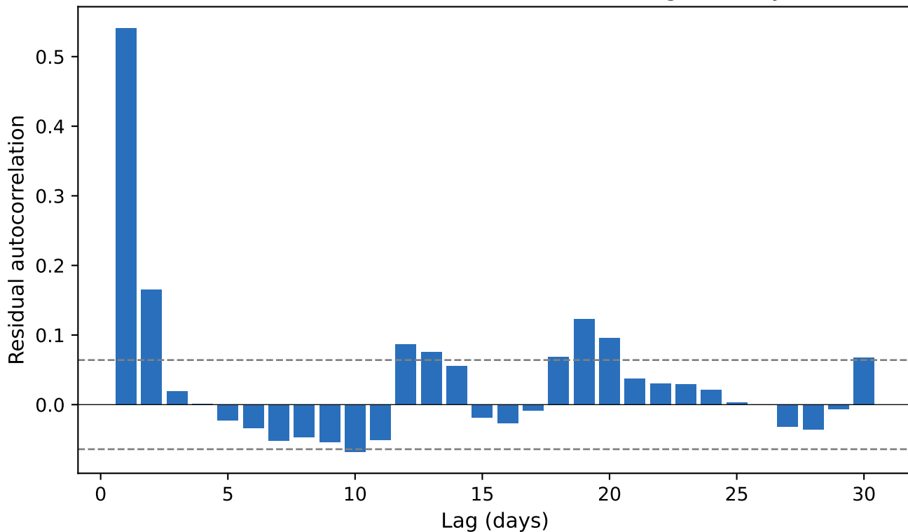
Baseline residual autocorrelation through 30 days
