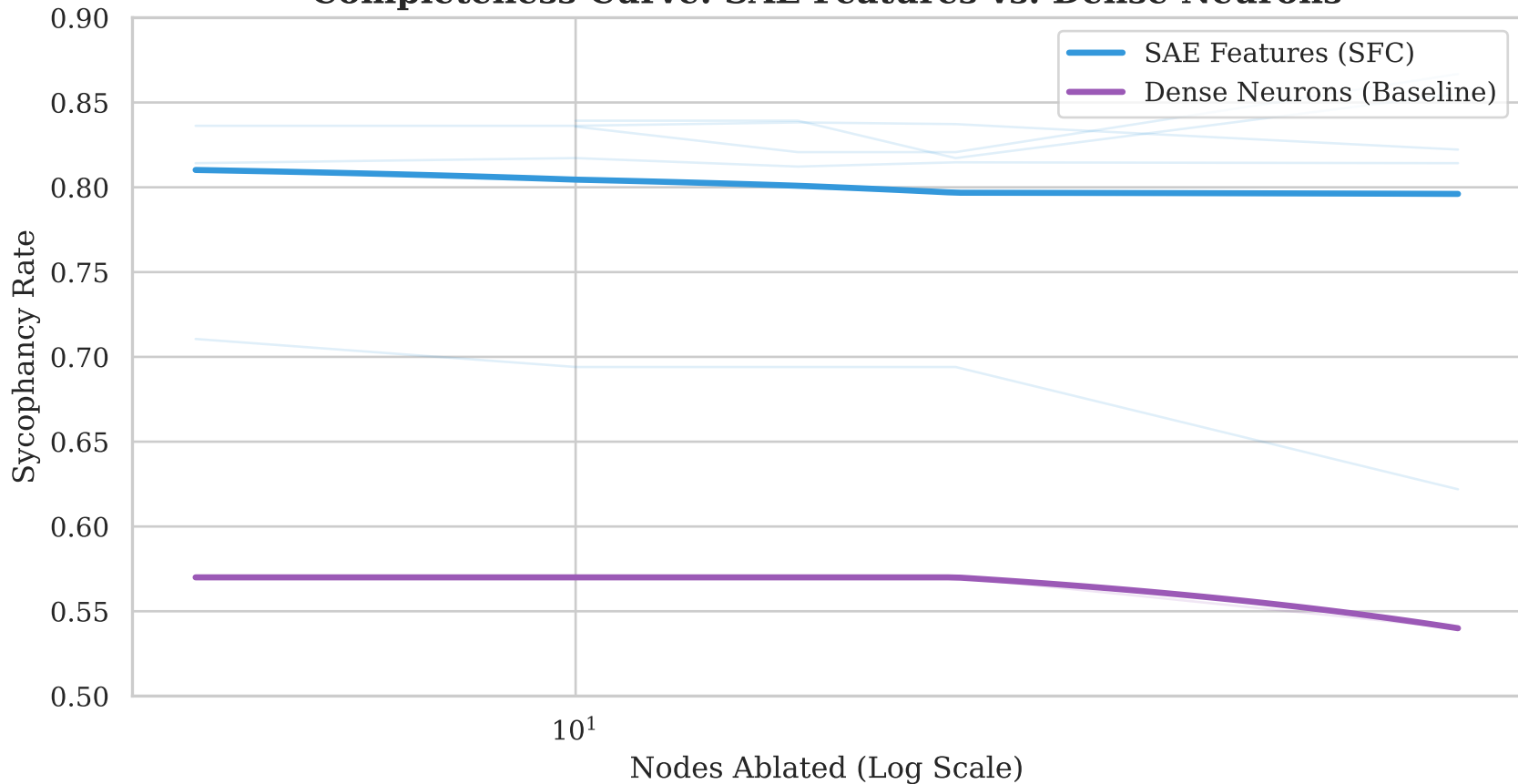
Completeness Curve: SAE Features vs. Dense Neurons
