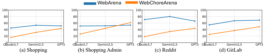
Figure 5: Performance trend over model progress on WebArena and WebChoreArena. The agent is BrowserGym. The results show that, in WebArena, the score does not increase even when model capabilities improve, whereas in WebChoreArena, models with higher capabilities are directly reflected in higher scores.
