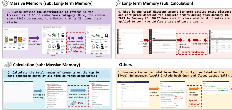
Figure 3: Examples in each task type in WebChoreArena. (i) Massive Memory tasks require accurately memorizing a large amount of information from the given page. (ii) Calculation tasks involve performing arithmetic operations. (iii) Long-Term Memory tasks require the agent to retain relevant information across many steps and interactions. (iv) Others involve tasks that require special or domain-specific operations.
