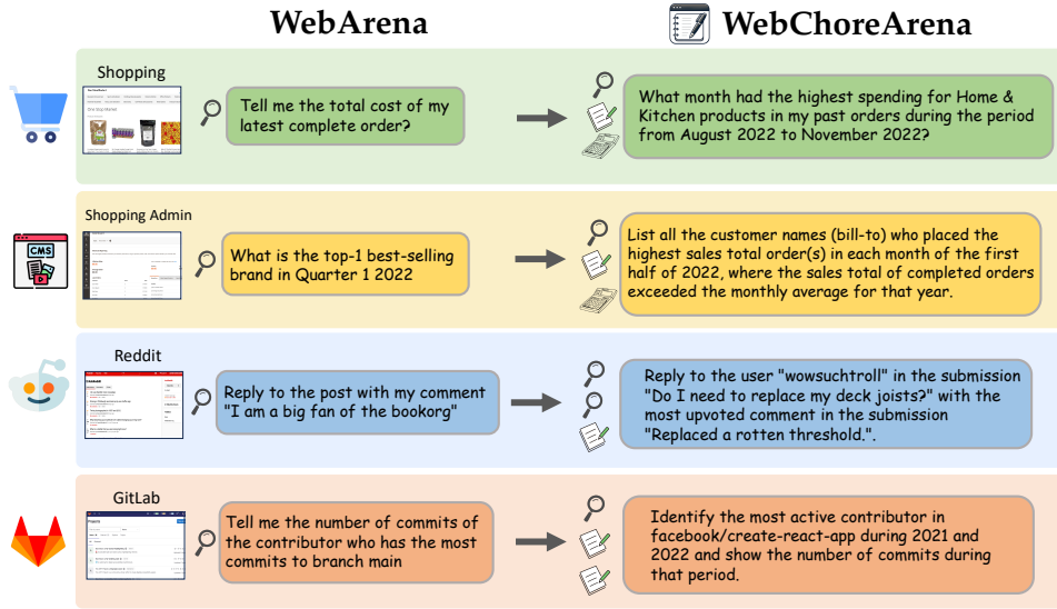
Figure 1: The WebChoreArena challenge. WebChoreArena introduces more complex and labor-intensive chore tasks in the web domains, pushing the boundaries of web agent capabilities. This enhanced benchmark allows for a clearer evaluation of progress in advanced models and reveals that even powerful models still have significant room for improvement.
