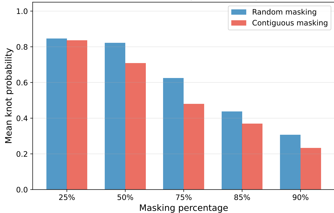
Random vs Contiguous Masking
