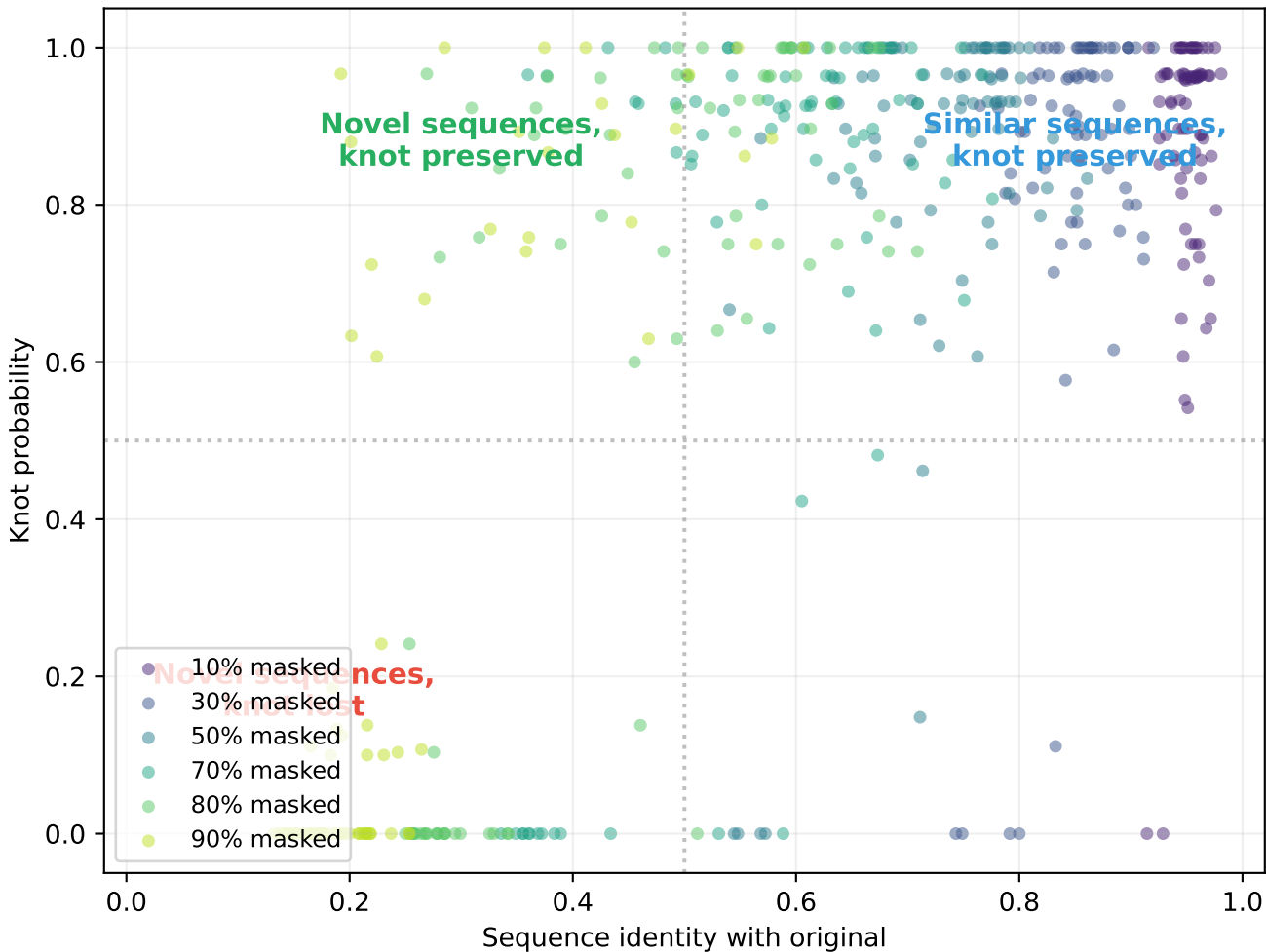
Sequence Novelty vs Topological Preservation
