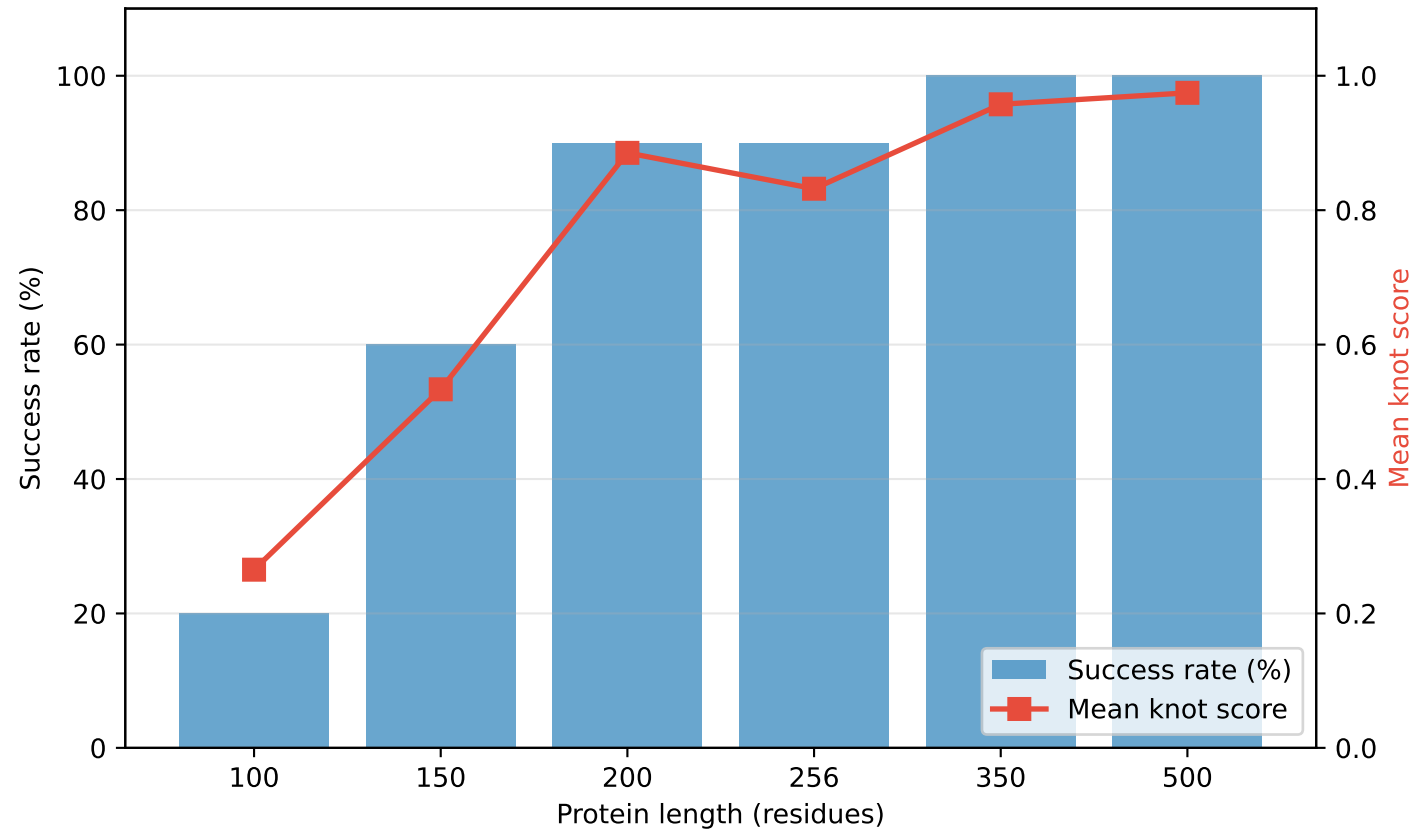
Guided Generation Success Rate by Protein Length (n=10 per length)
