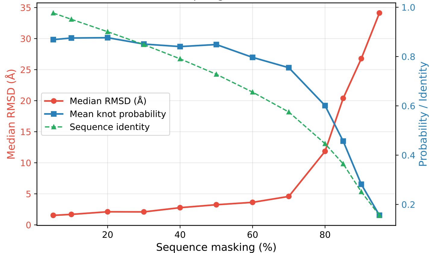
Structural Drift vs Topological Persistence (n=80)
