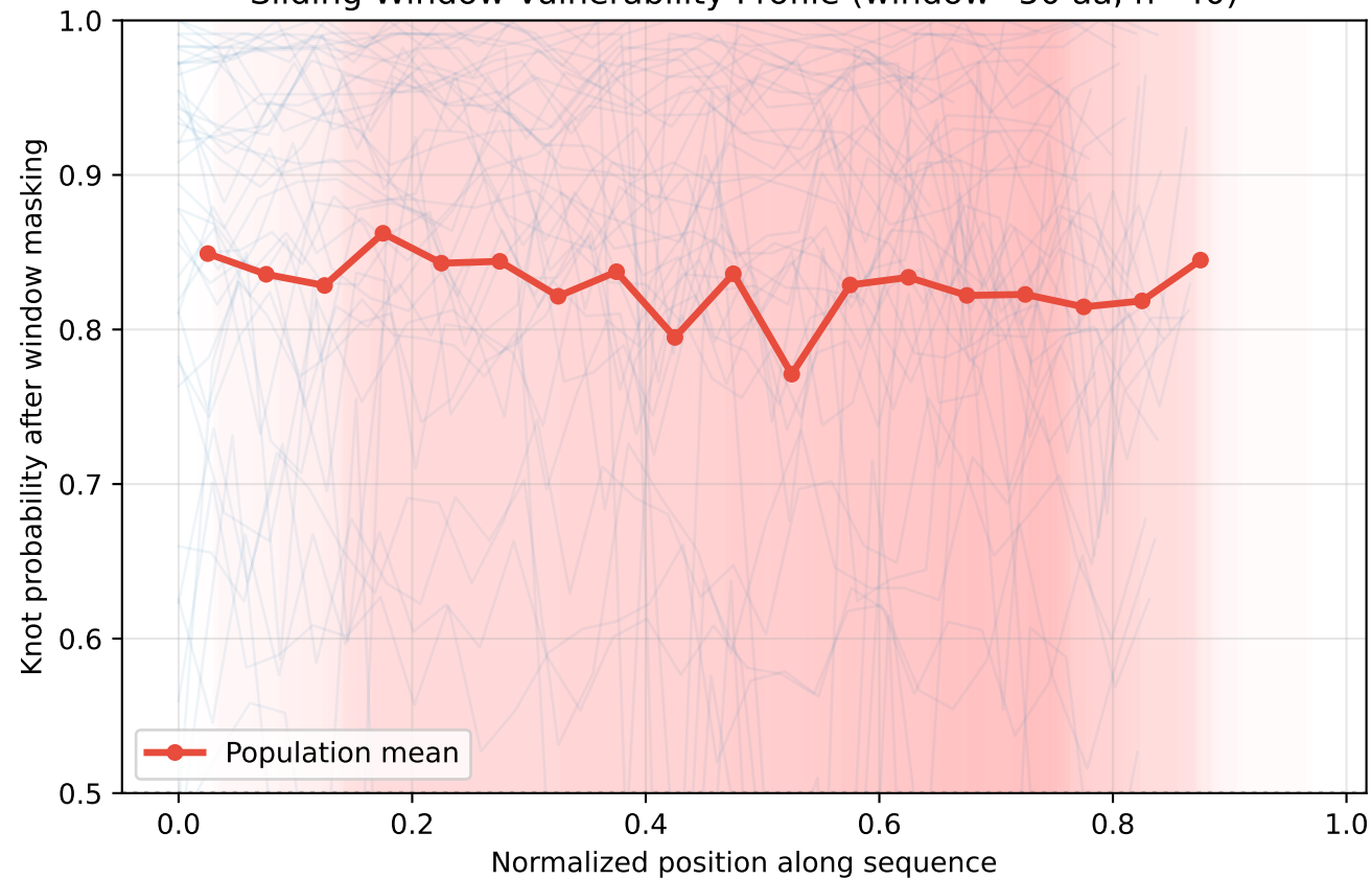
Sliding Window Vulnerability Profile (window=50 aa, n=40)
