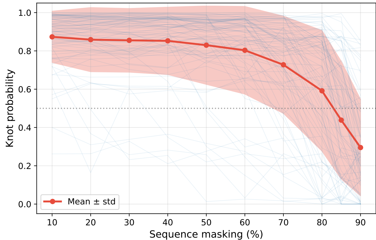
Individual Protein Transition Curves (n=80)
