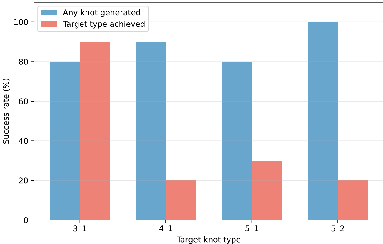
Knot-Type-Specific Guided Generation (n=10 per type, length=300)
