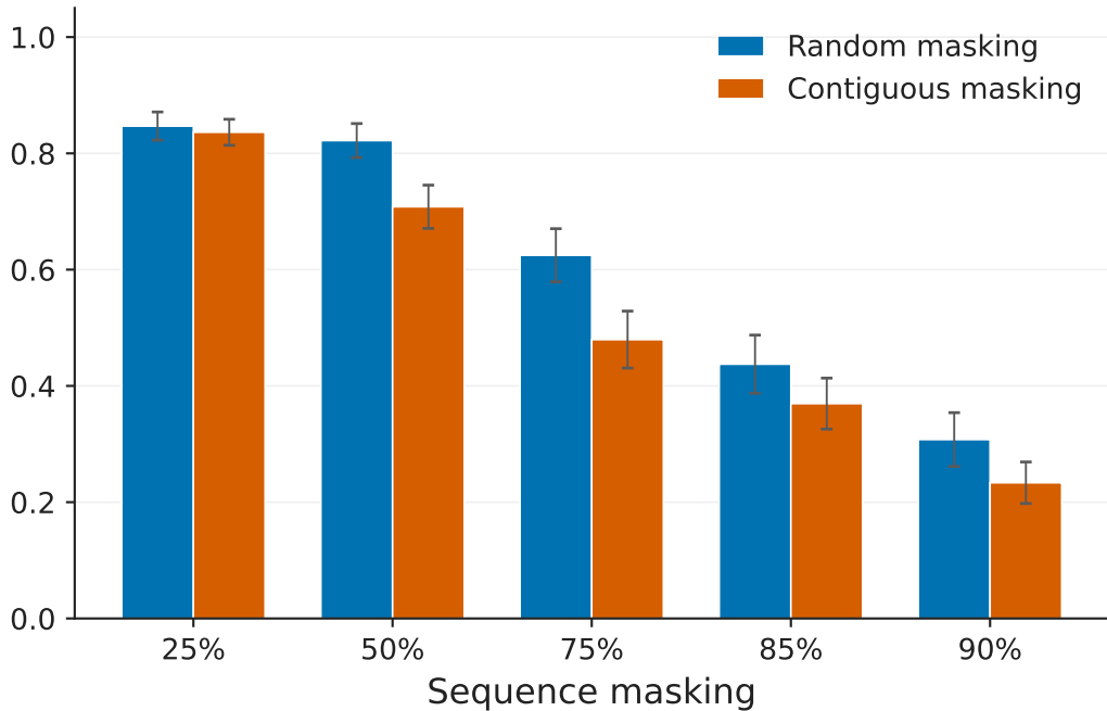
Mean knot probability
